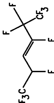
(3Z)-1,1,1,2,2,3,5,5,6,6,6-decafluorohex-3-ene
