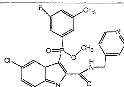
Compound P
