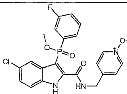
Compound I
