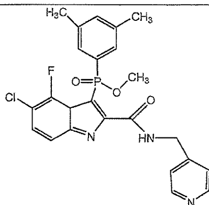
Compound M
