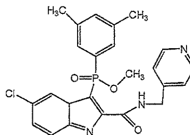
Compound N
