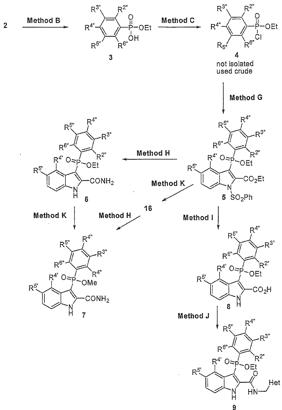
Scheme 3:
