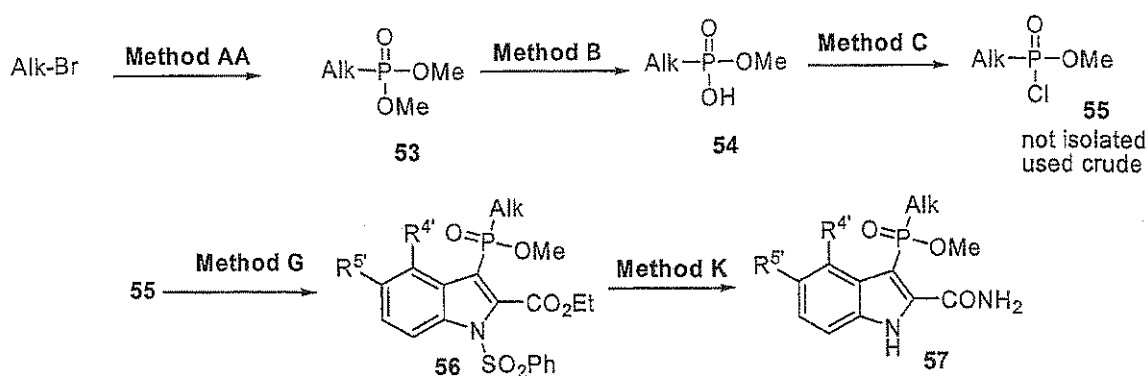
Scheme 14: Alkyl Phosphinates
