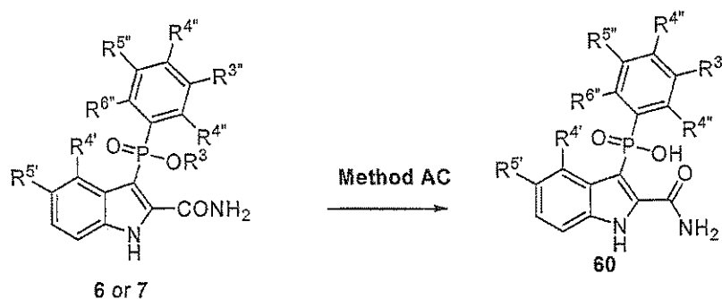
Scheme 16: Phosphinic Acids
