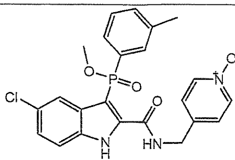
Compound J
