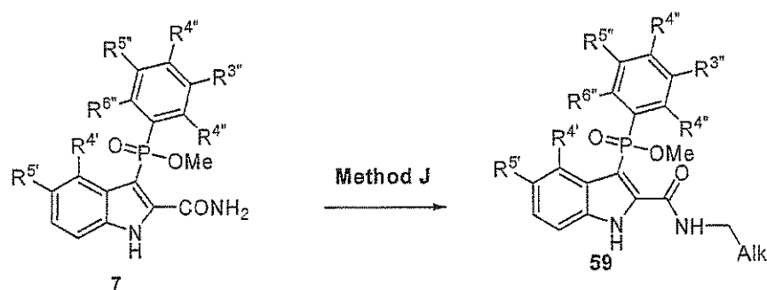
Scheme 16: Phosphinic Acids
