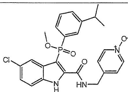
Compound M
