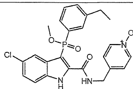
Compound L
