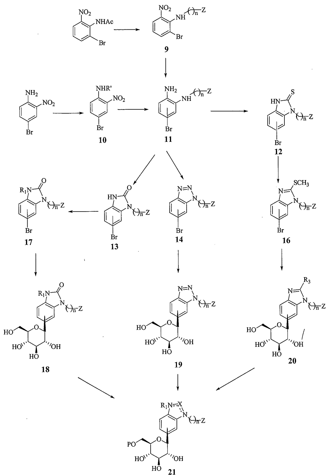
Scheme 2
