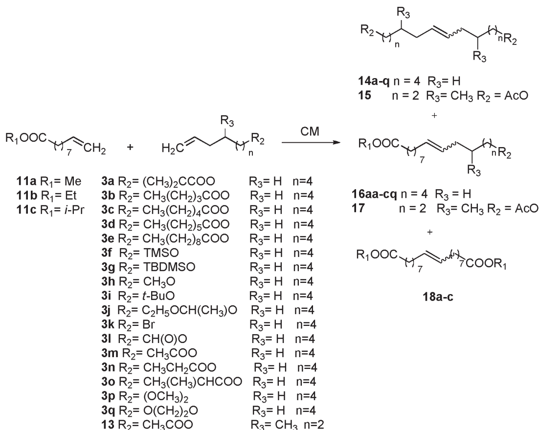
Scheme 2. Cross metathesis of decenoic acid esters ( 11a-c ) with oct-7-enol and 3-methylhex-5-enol ( 3a-q and 13 ).
