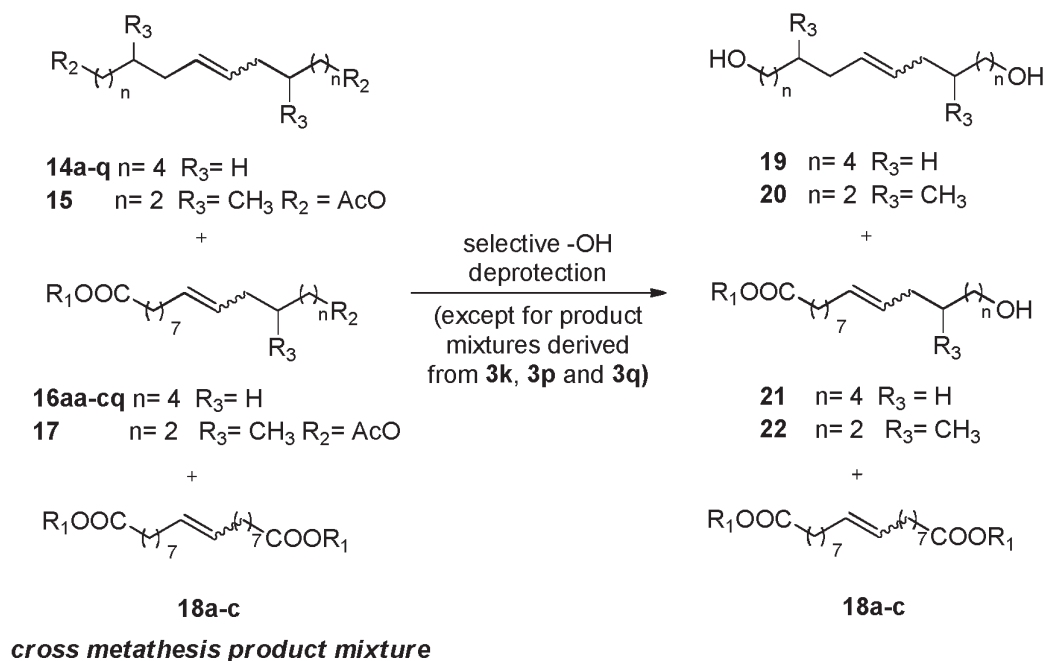
Scheme 4. Synthesis of \omega -hydroxy esters ( 21a-c , 22 ).
