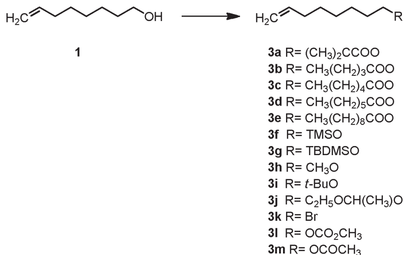
Scheme 1. Synthesis of oct-7-enol derivatives.
