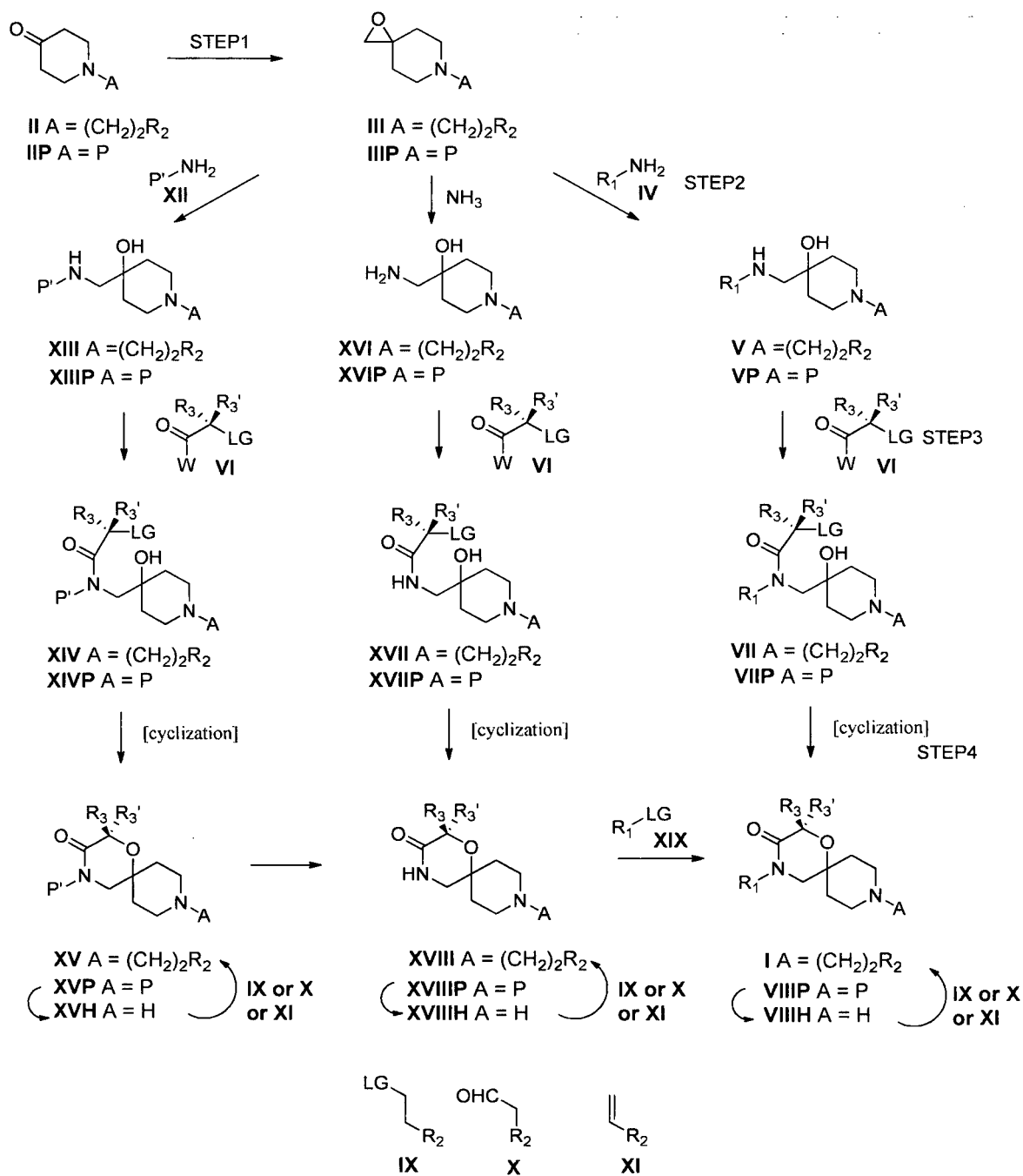
Scheme 1
