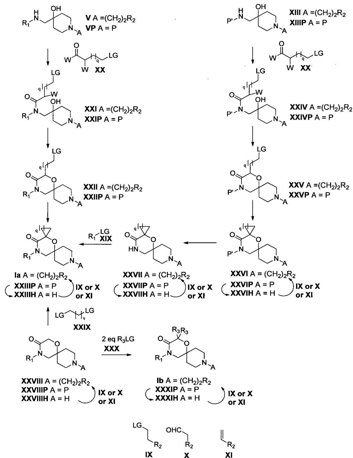
Scheme 2
