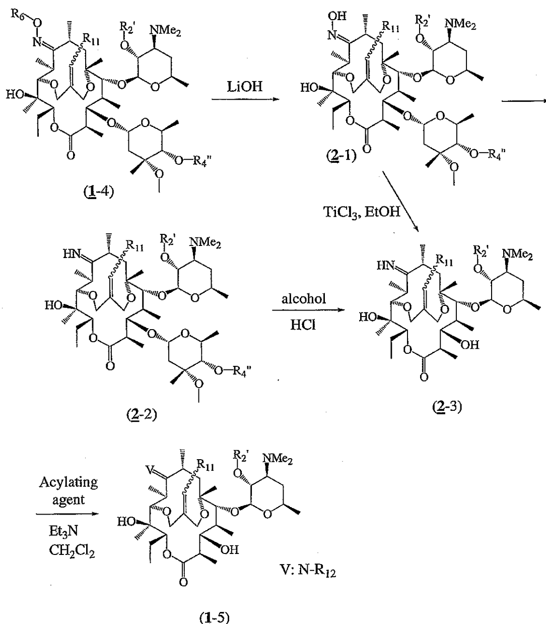
Scheme 2
