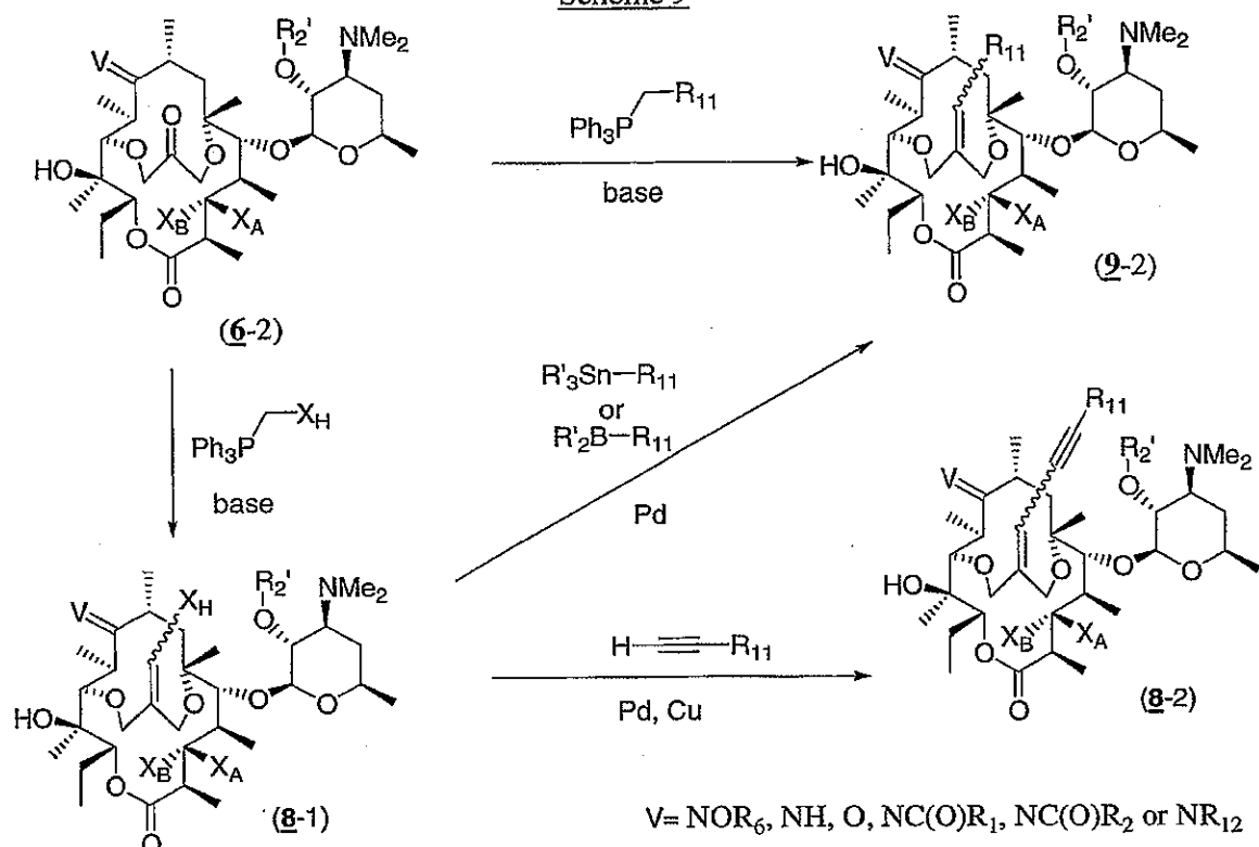
Scheme 9
