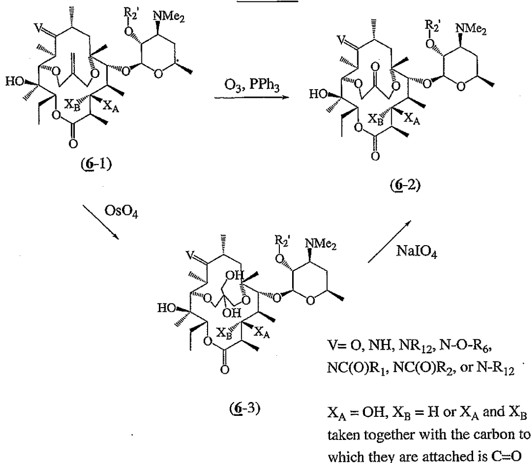
Scheme 5
