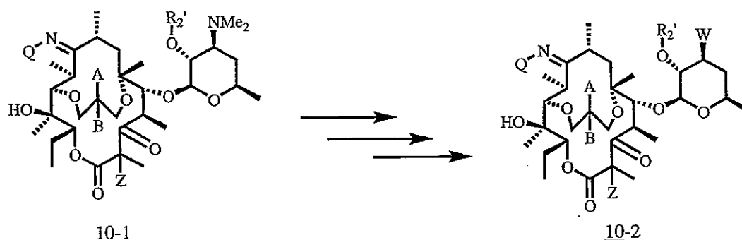
Scheme 10
