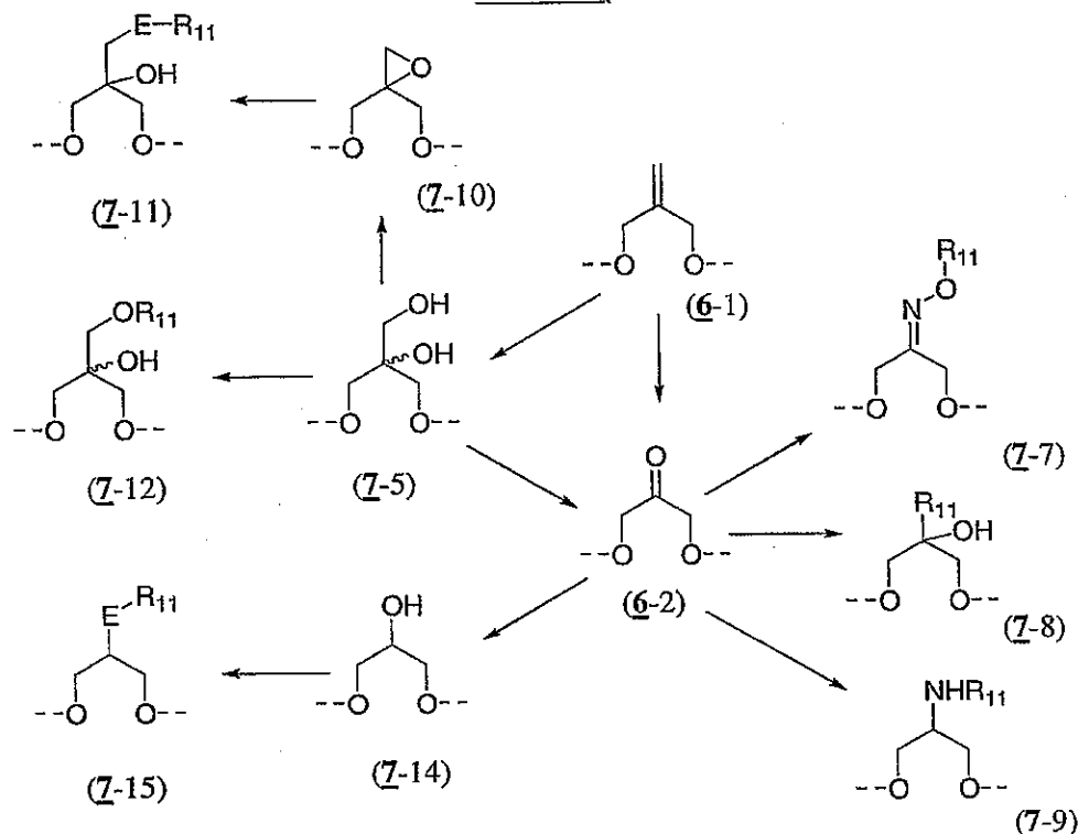
Scheme 7.
