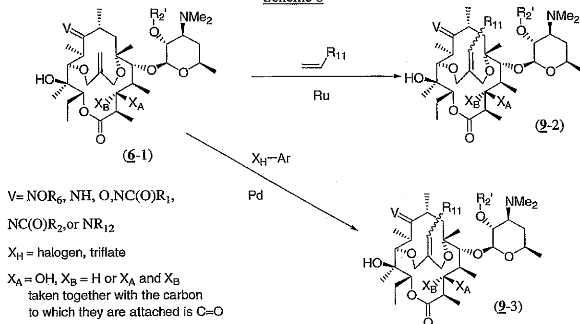
Scheme 8
