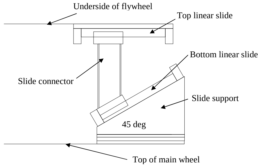
Side View of a simplified sliding angular coupling
