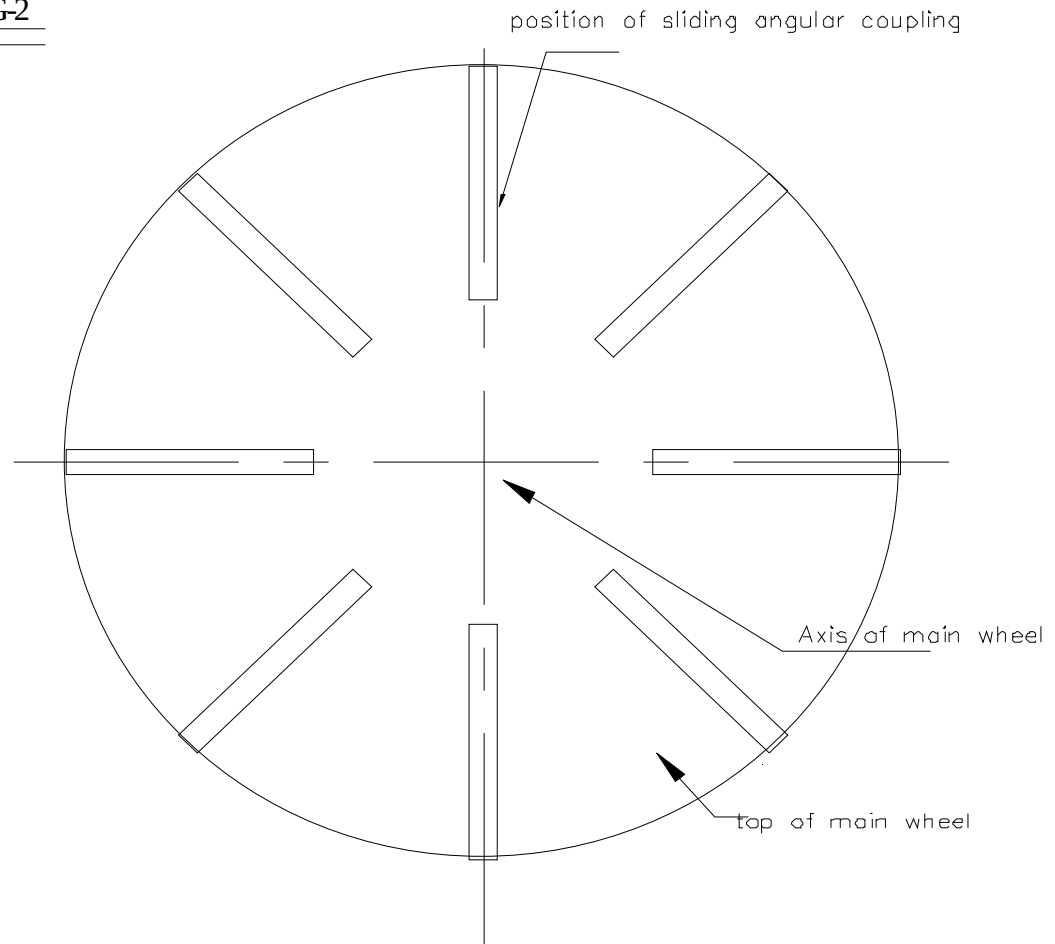
Plan layout of sliding angular coupling on top of main wheel
