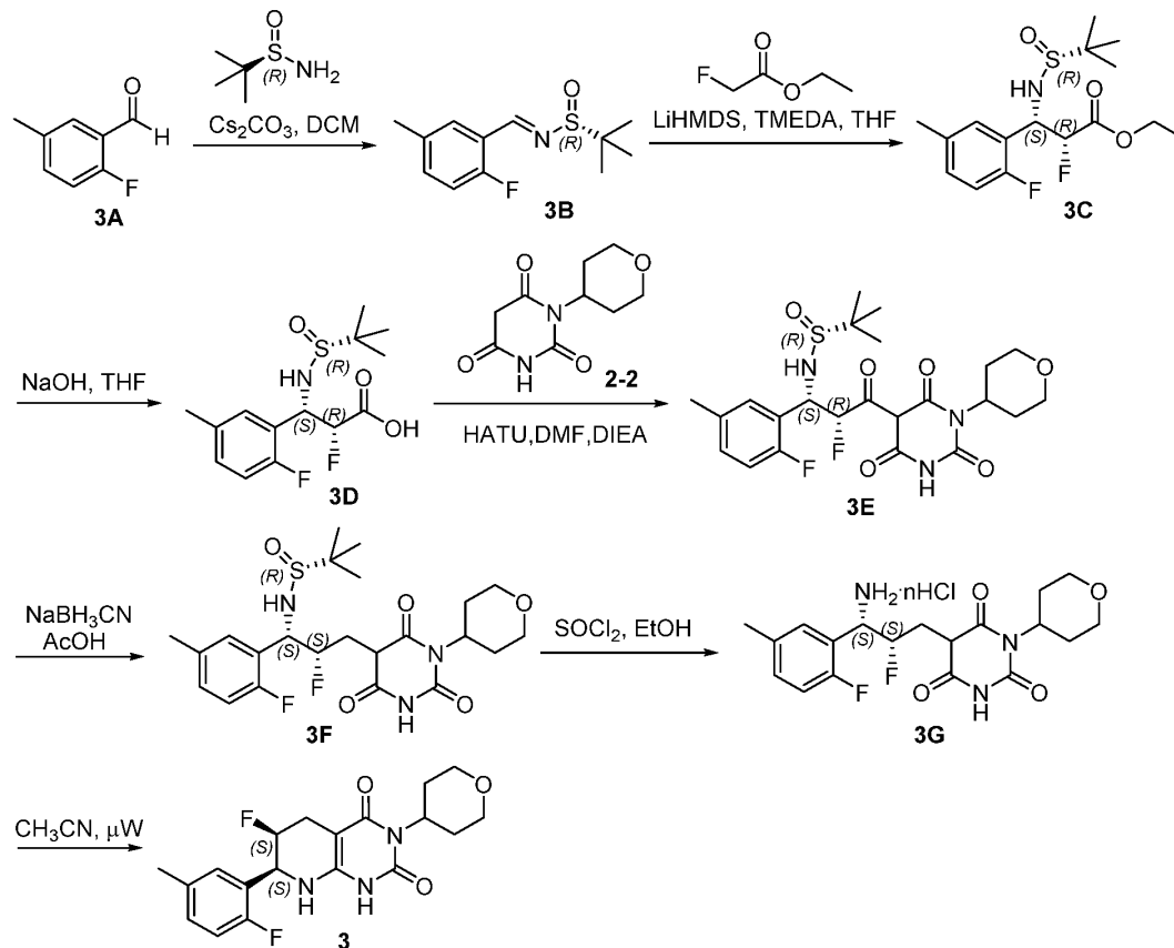
Scheme 3
