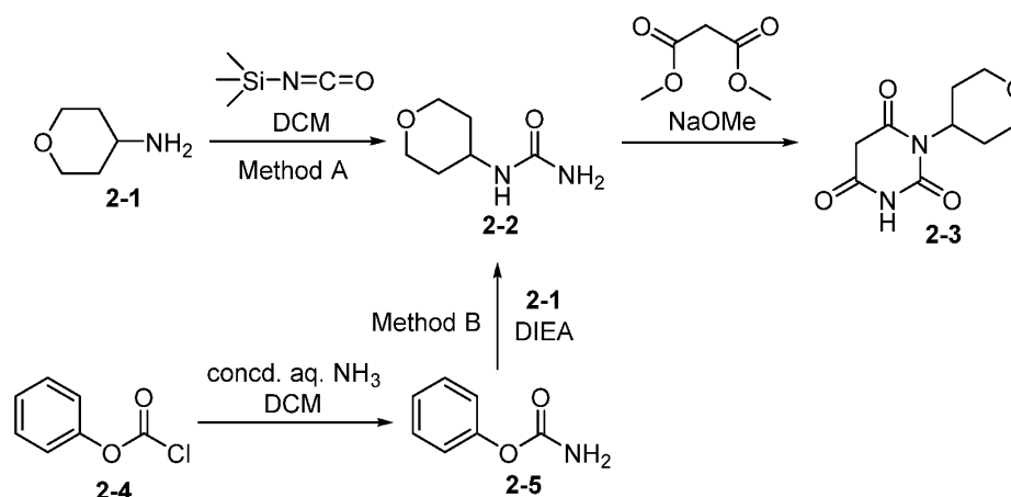
Scheme I-2
