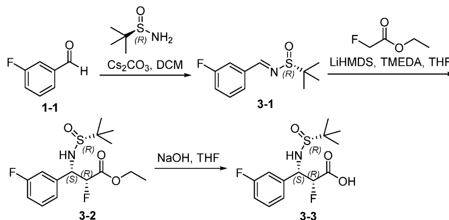
Scheme I-3
