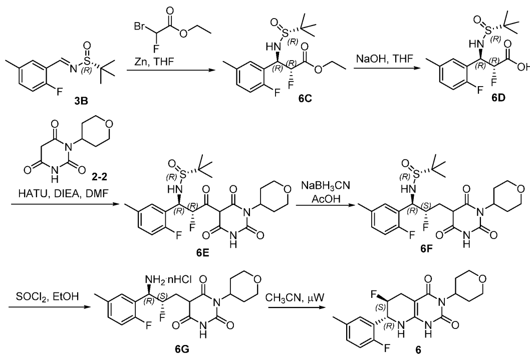
Scheme 6
