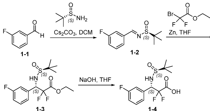
Scheme I-1
