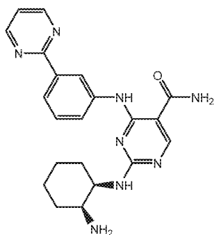
Compound 1,
