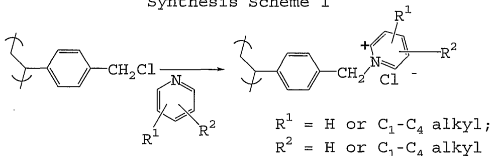
Synthesis Scheme 1
