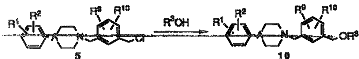
Reaction Scheme 3
