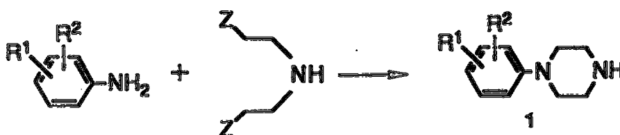
Reaction Scheme 4
