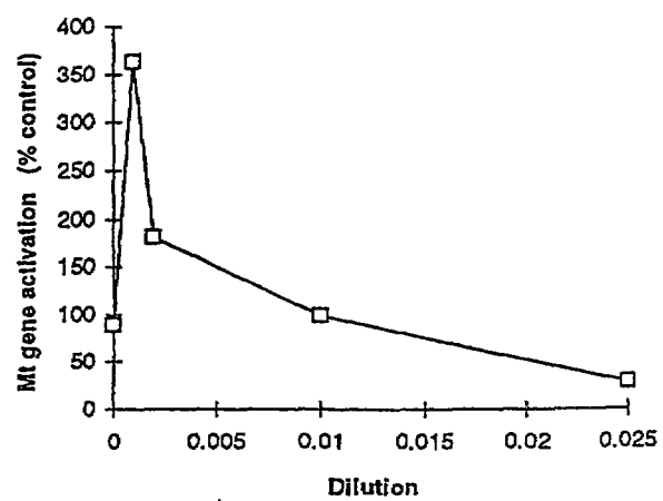
Effect of Substance A on metallothionein gene activation
