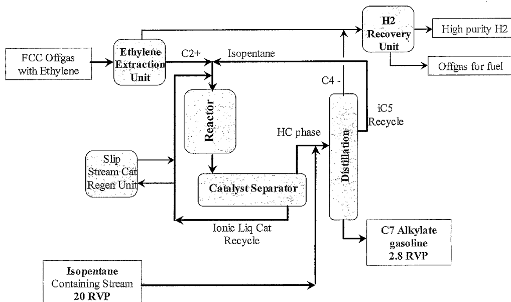
Isopentane and Ethylene Alkylation Process Scheme
