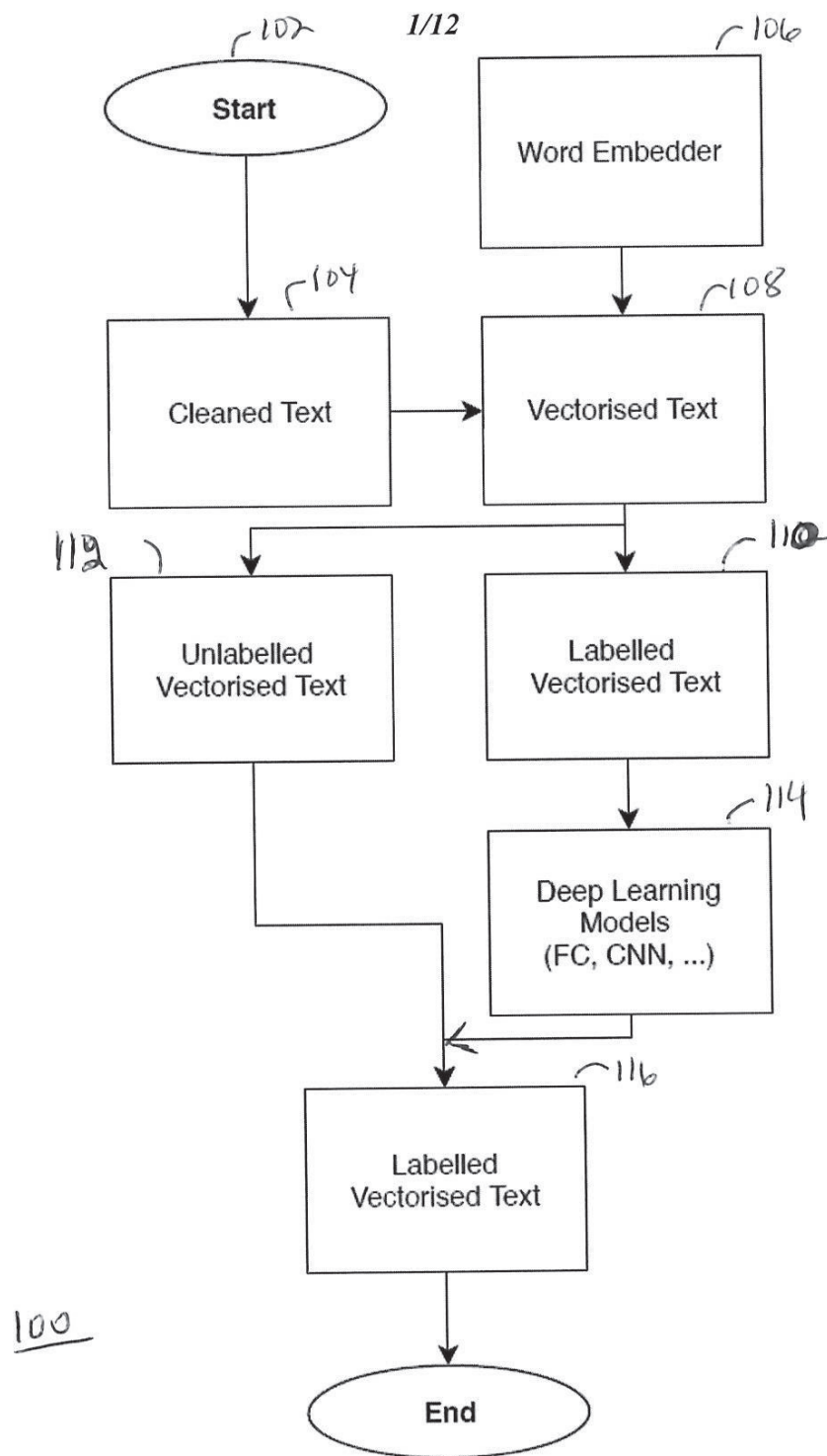
a) First prediction of documents and construction of the model
