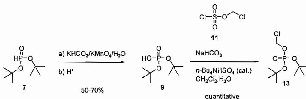
Scheme (III)
