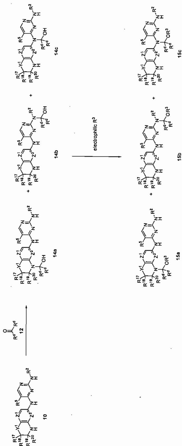
Scheme (I)
