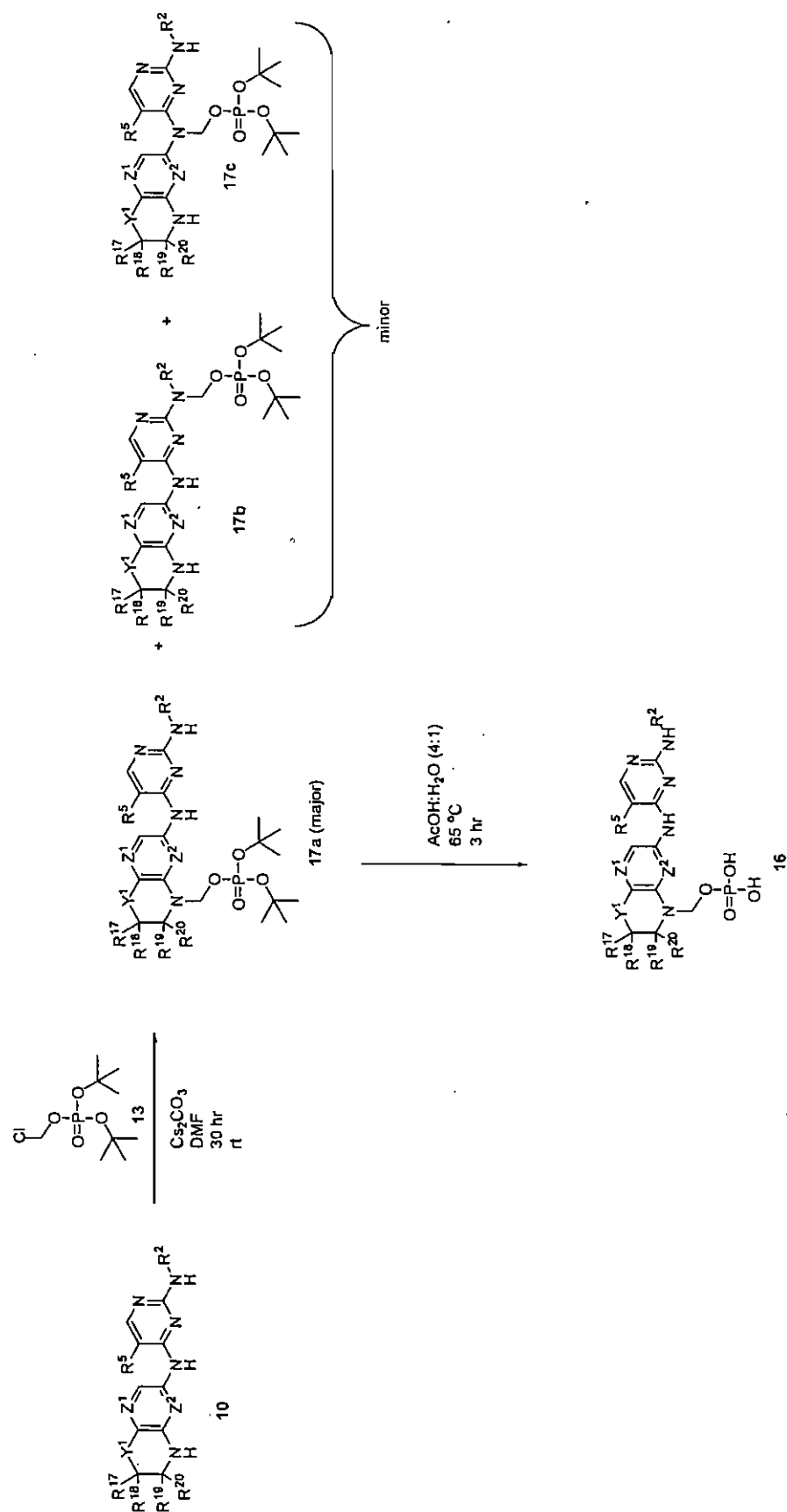
Scheme (V)
