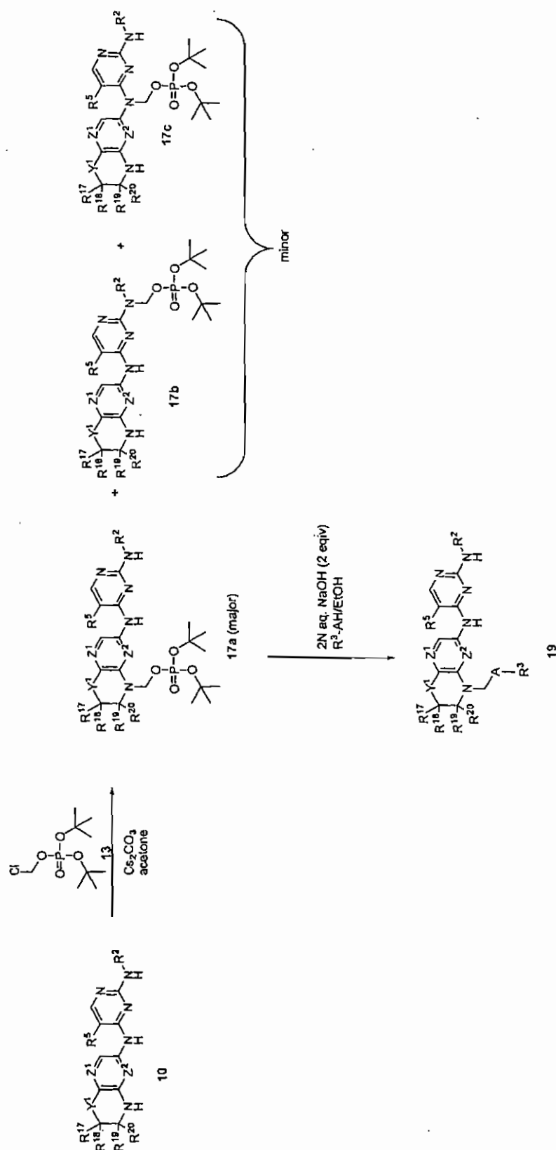
Scheme II
