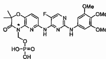
Compound 4
