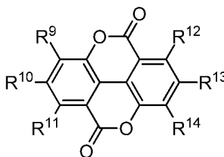
Formula VI
