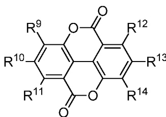
Formula IV
