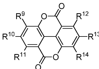
Formula VI
