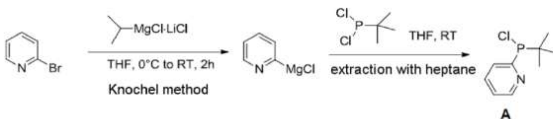
Scheme 1: Synthesis of precursor A
