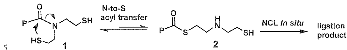
Scheme 2. N -to- S acyl transfer using an N,N -di-(2-mercaptoethyl)-substituted tertiary amide to generate thioester peptides for NCL.
