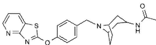
JNJ-40929837
