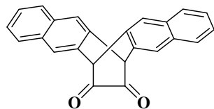
Compound B
