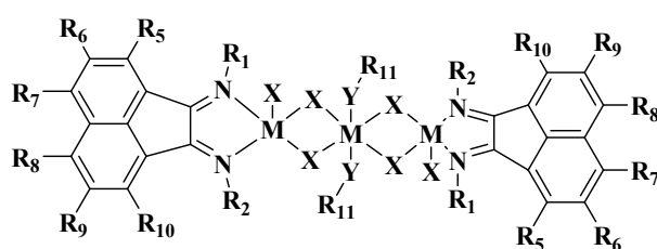
Formula IIa
