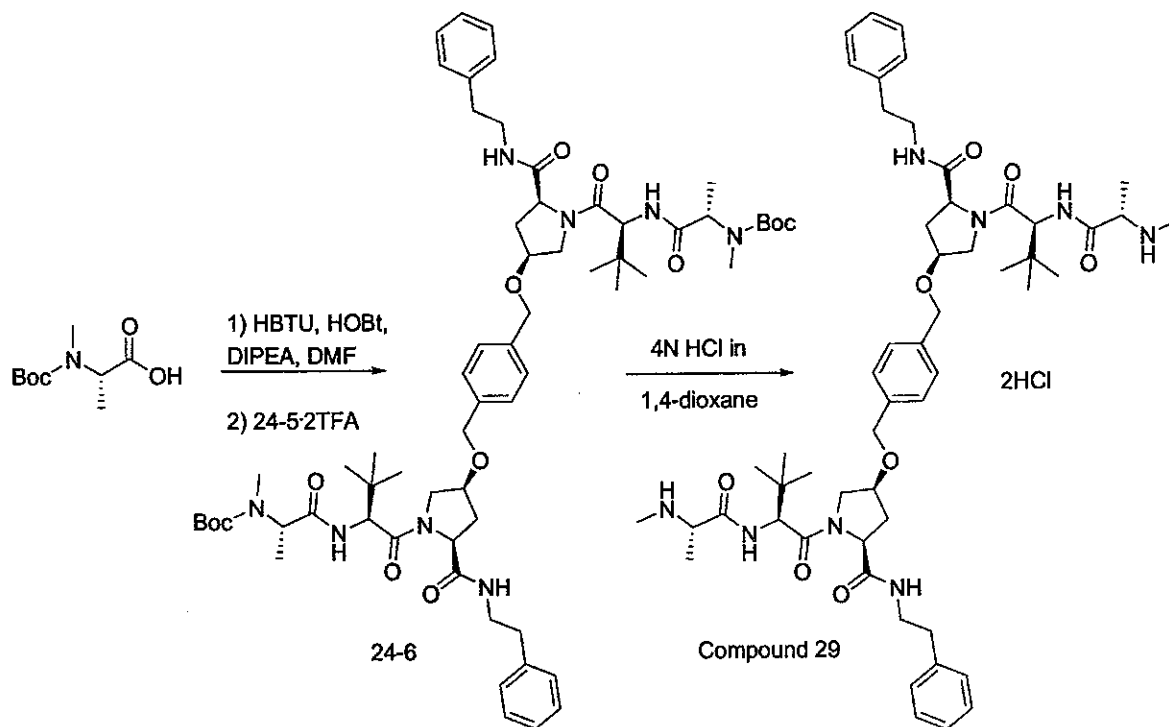
Scheme 24
