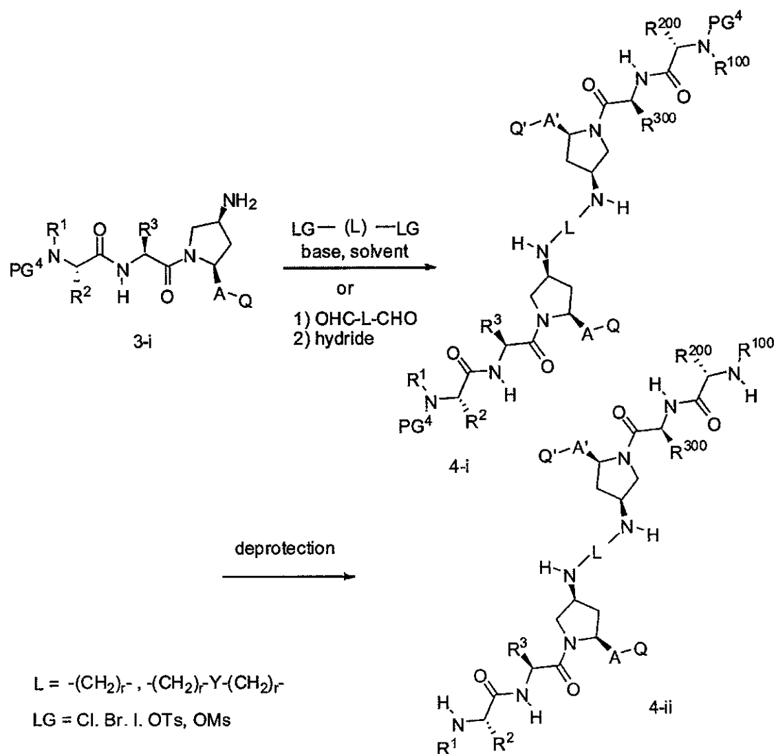
Scheme 4
