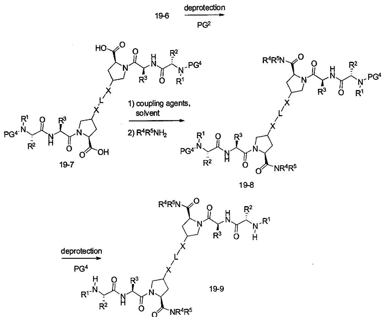
Scheme 19b
