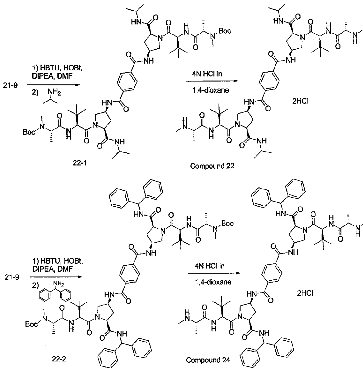
Scheme 22
