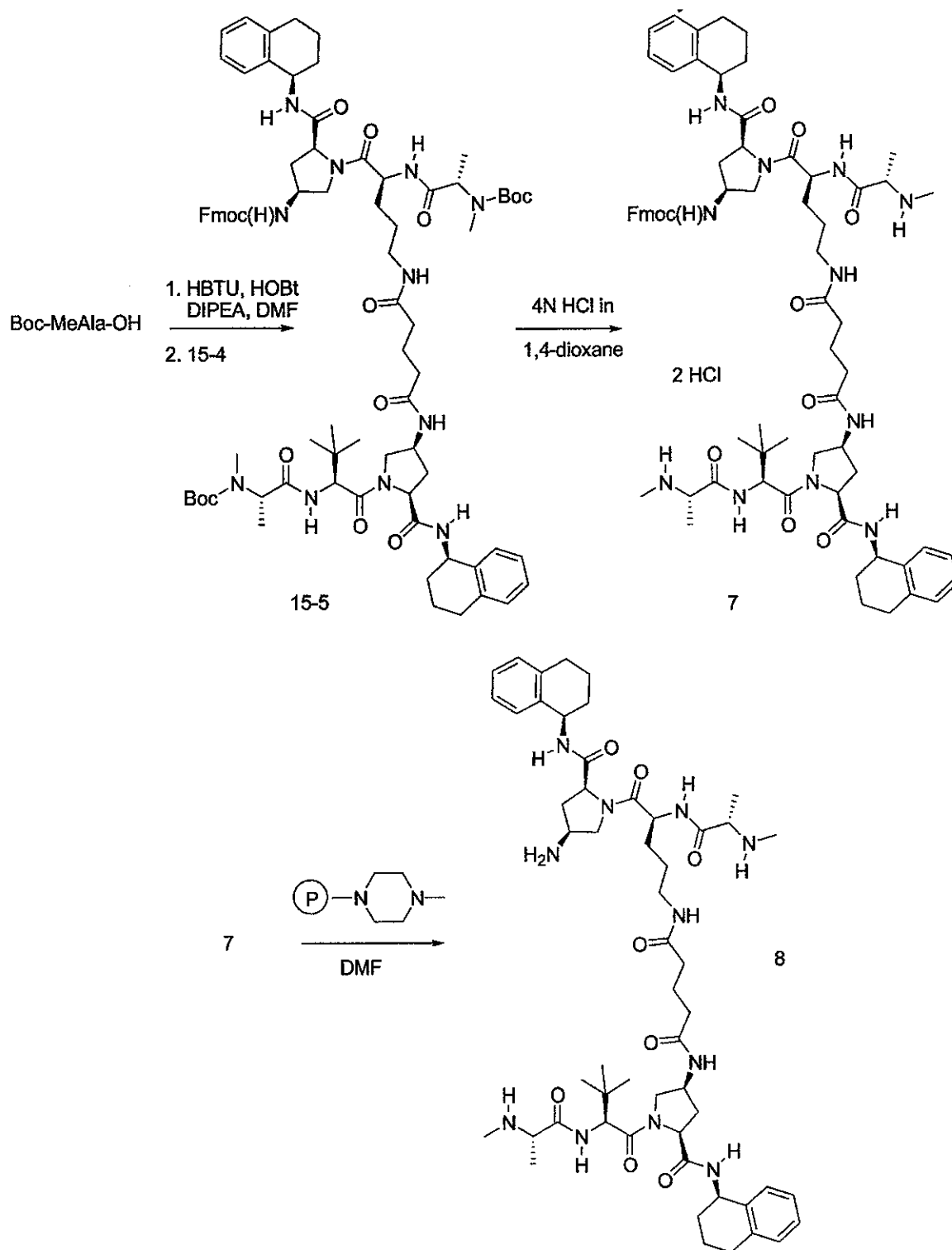
Scheme 15
