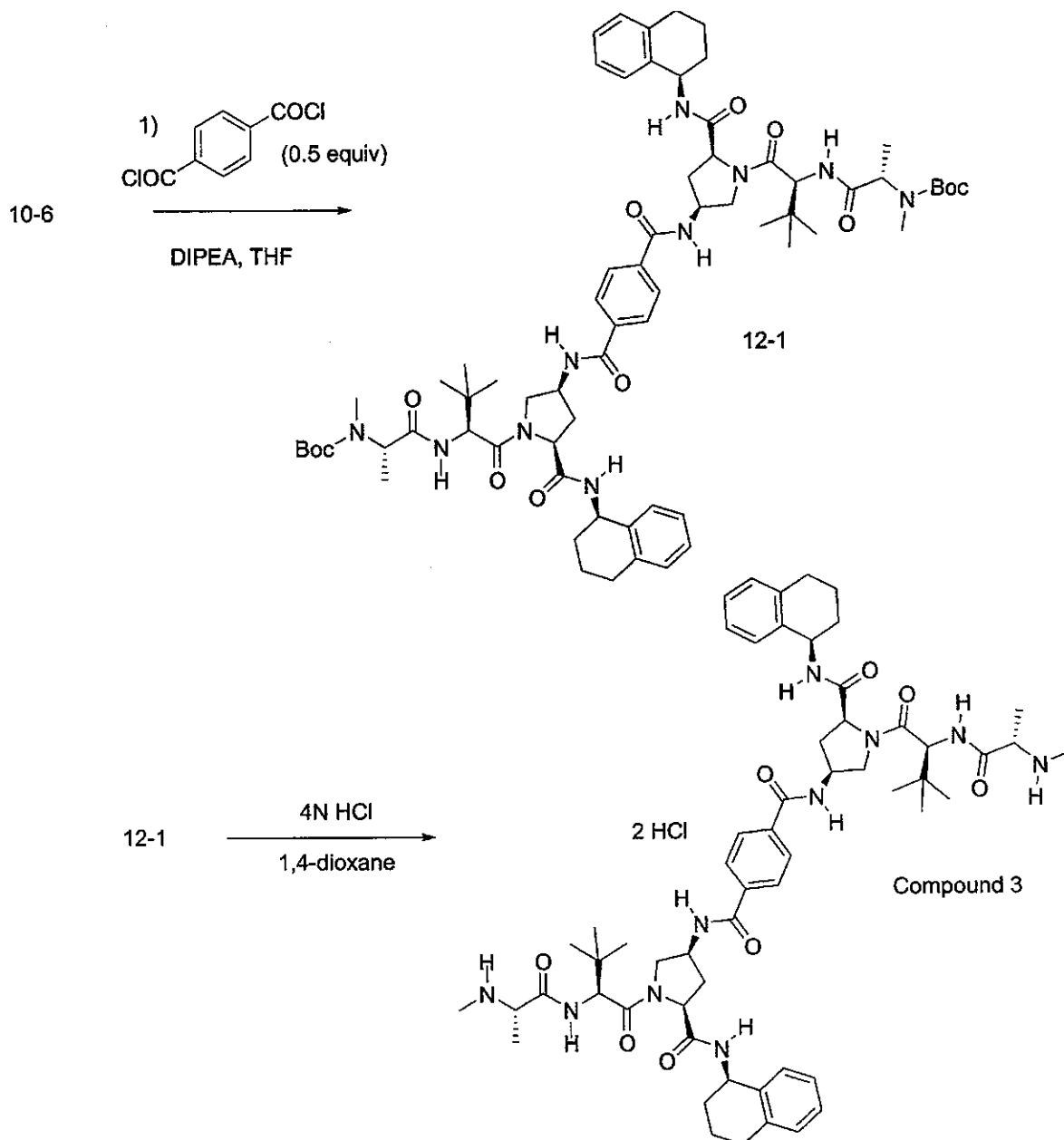
Scheme 12
