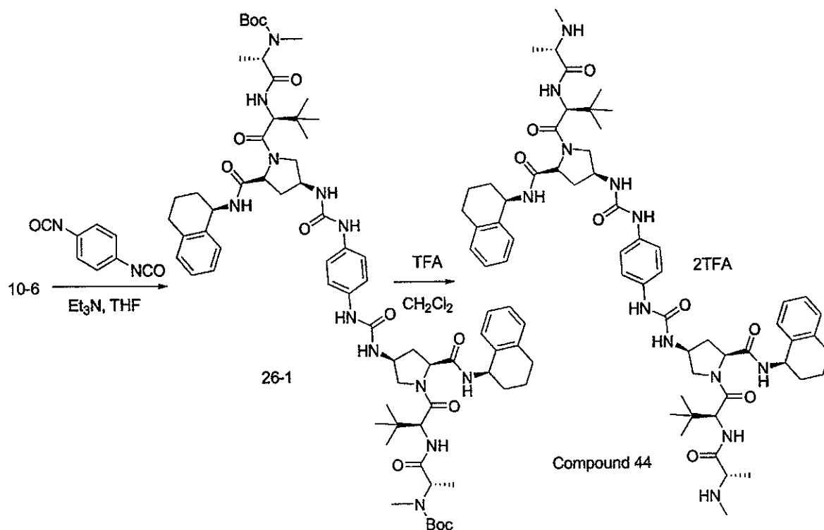
Scheme 26
