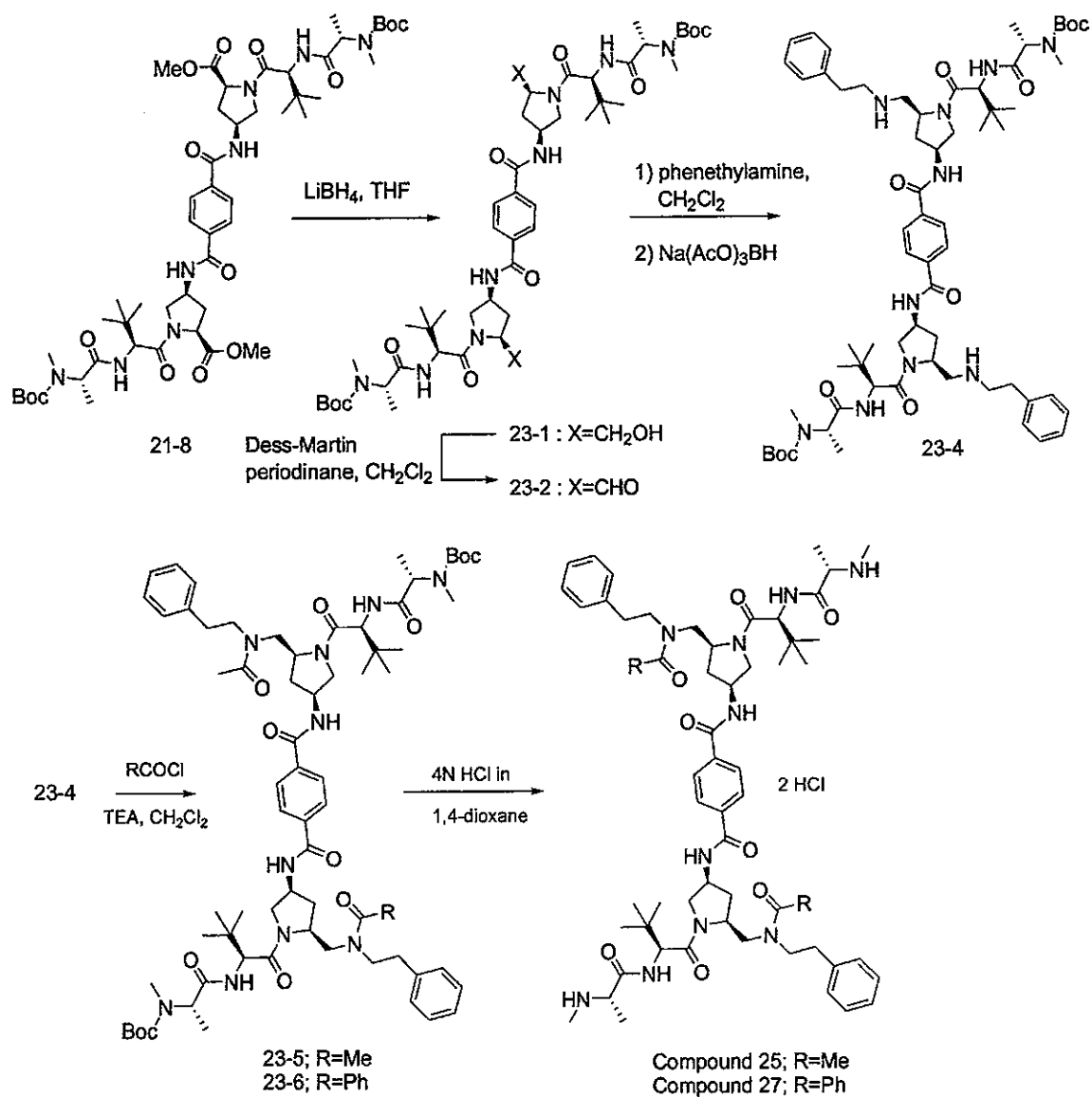
Scheme 23a
