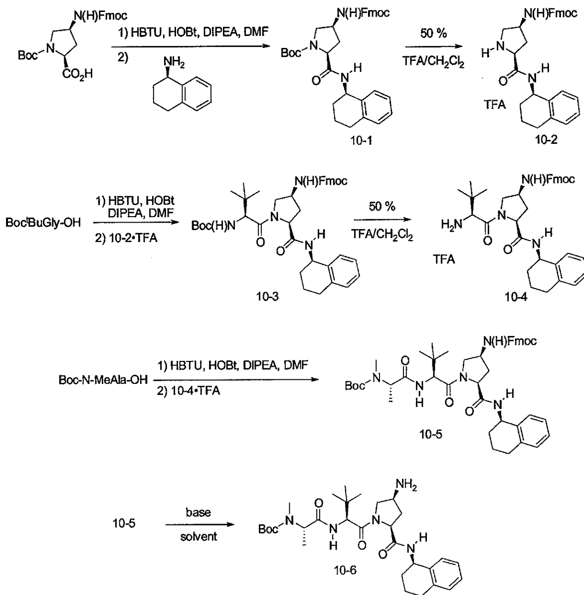
Scheme 10
