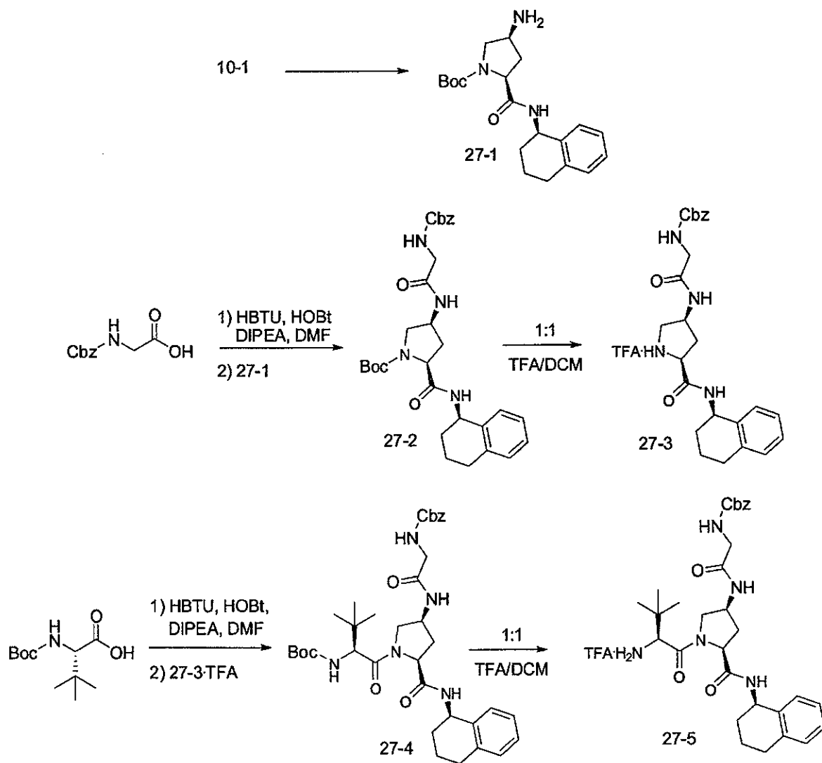
Scheme 27a
