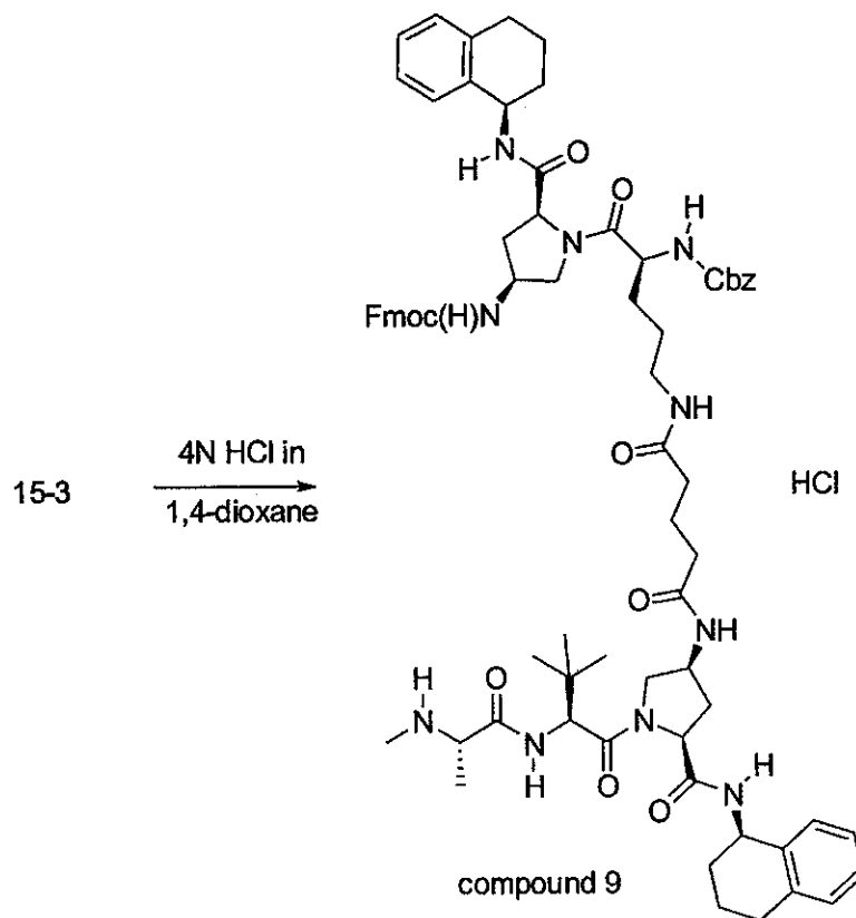
Scheme 16
