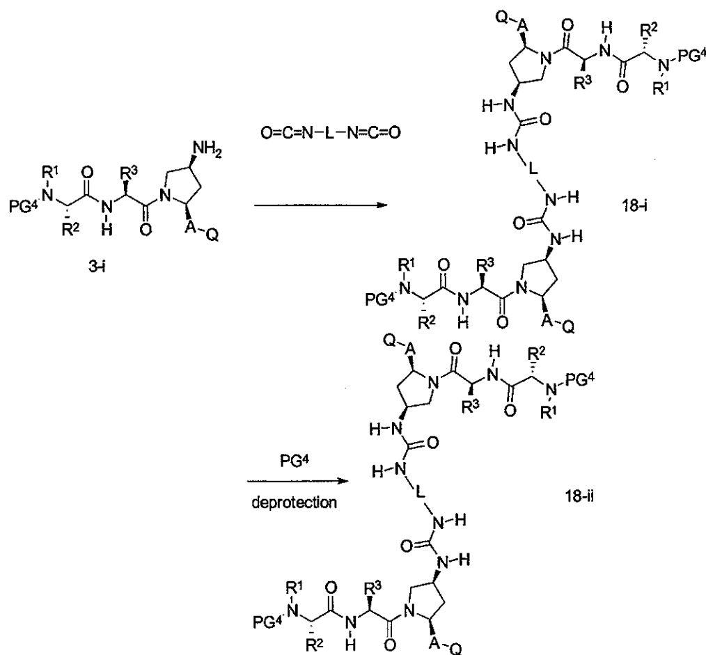
Scheme 18
