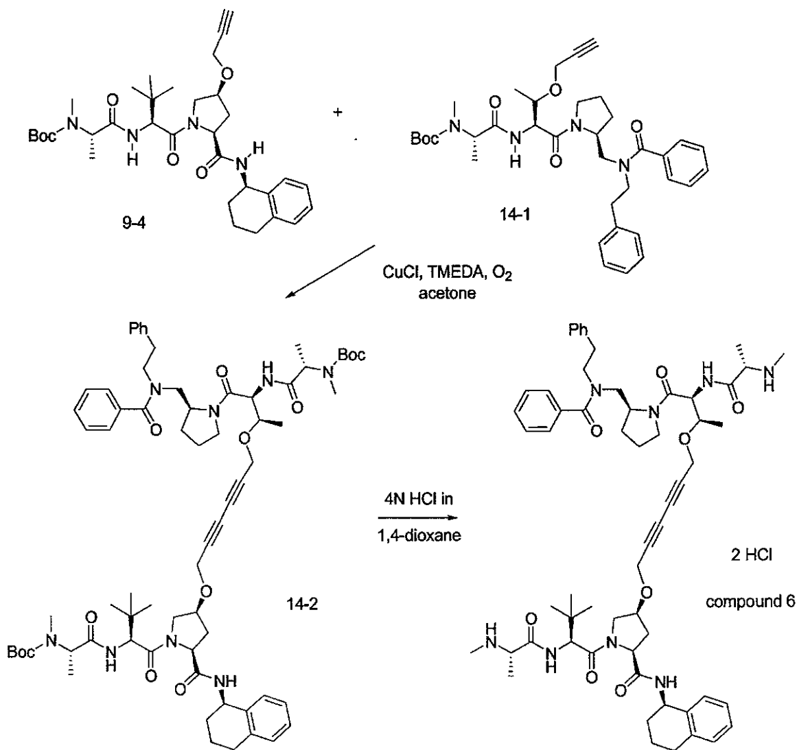
Scheme 14:
