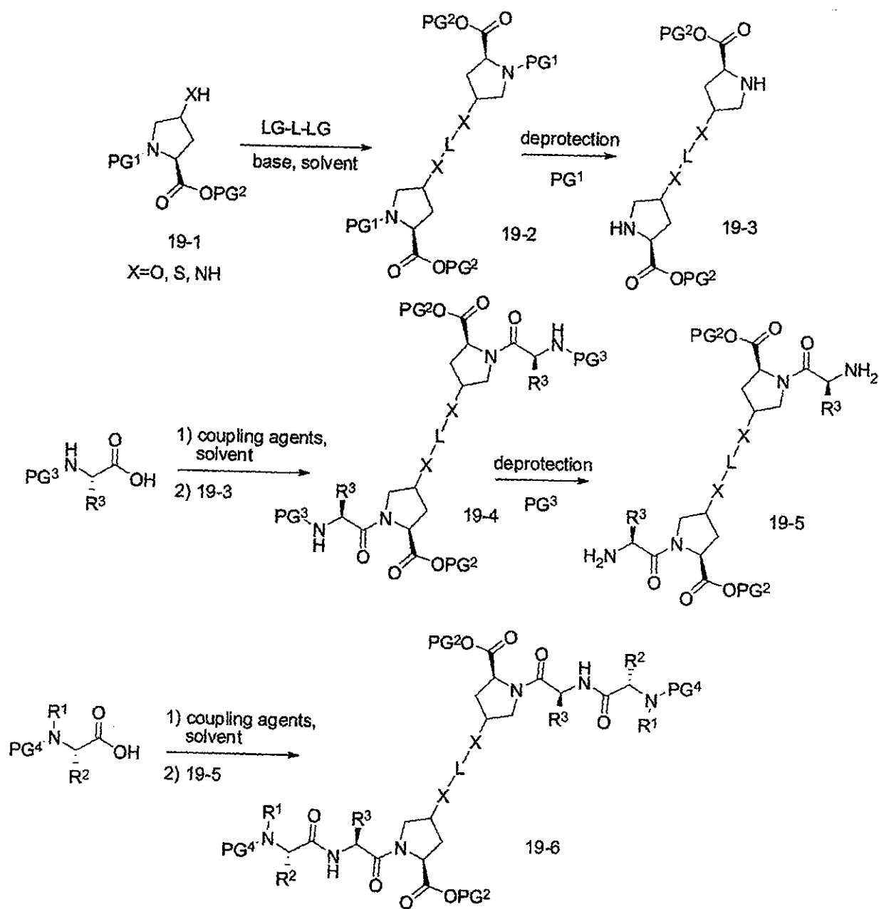
Scheme 19a
