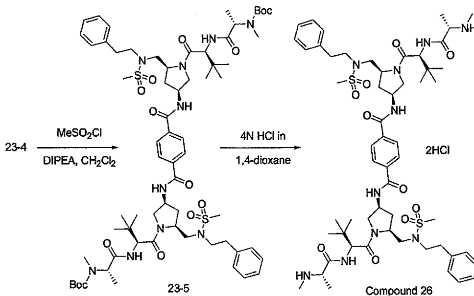
Scheme 23b
