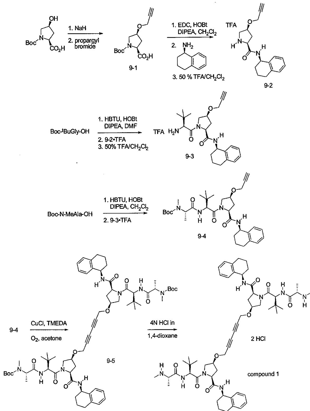
Scheme 9
