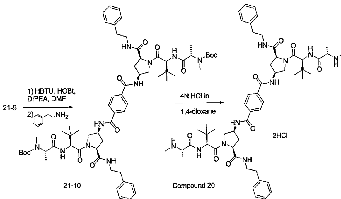
Scheme 21
