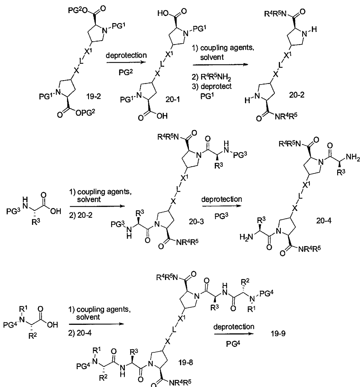
Scheme 20
