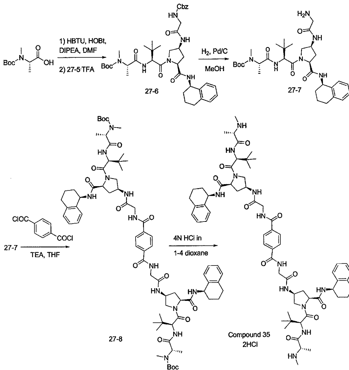
Scheme 27b
