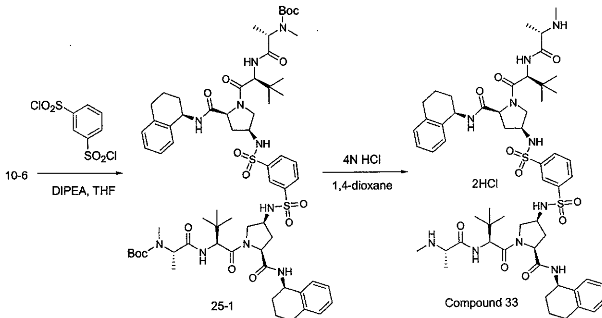
Scheme 25
