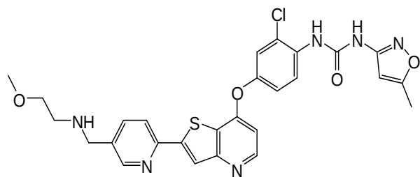
(Cpd. 298a, example 188a),
