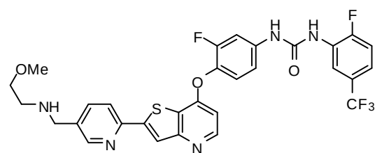
(Cpd. 253, example 146),
