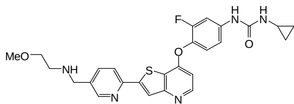
(Cpd. 277, example 170),
