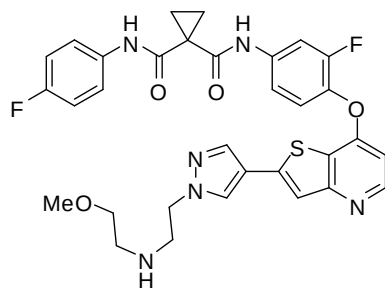
(Cpd. 82, example 25)
