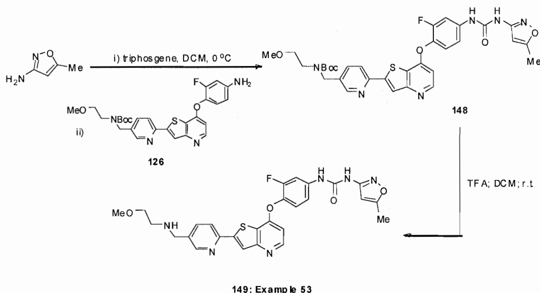
149: Example 53
