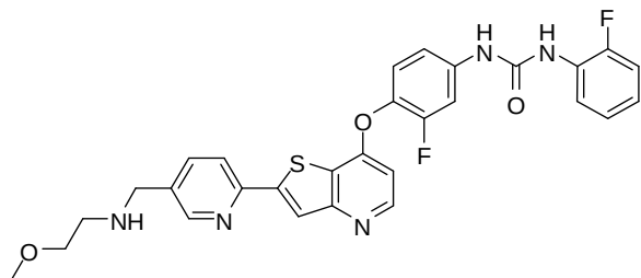
(Cpd. 332, example 218),
