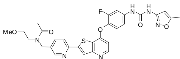
(Cpd. 339 example 225),
