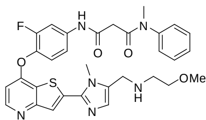
(Cpd. 50, example 14),
