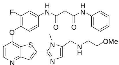
(Cpd. 49, example 13)
