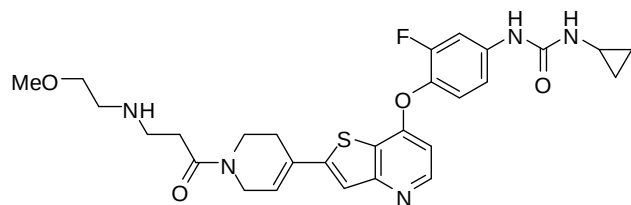
(Cpd. 352 example 238), and
