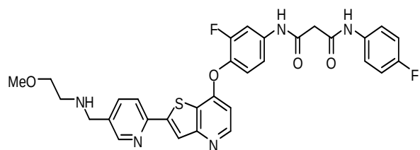
(Cpd. 237, example 130),
