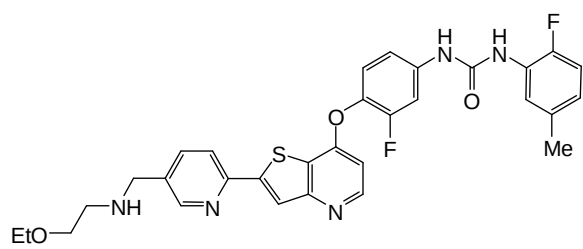
(Cpd. 280, example 173),
