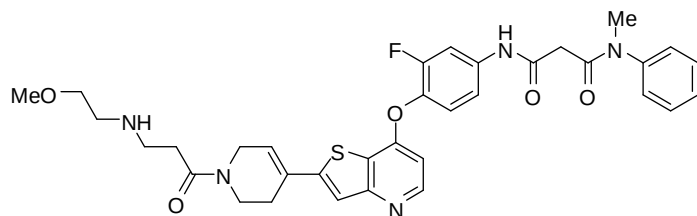
(Cpd. 102, example 33),
