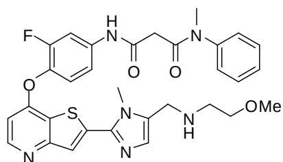
(Cpd. 50, example 14)
