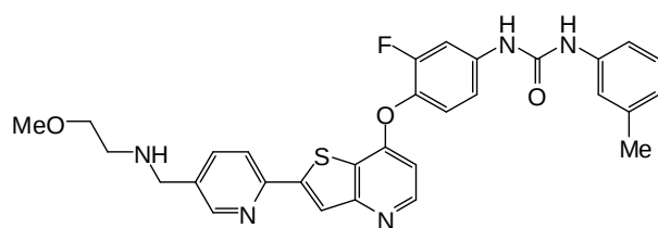
(Cpd. 268, example 161),
