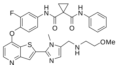
(Cpd. 51, example 15)
