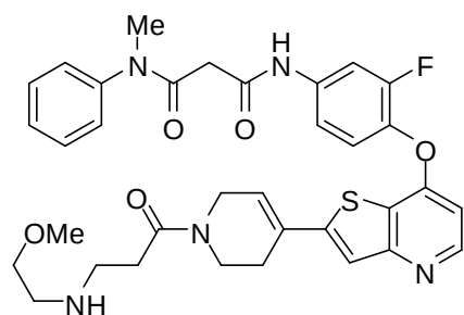
(Cpd. 102, example 33)
