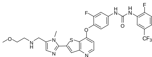
(Cpd. 344 example 230),
