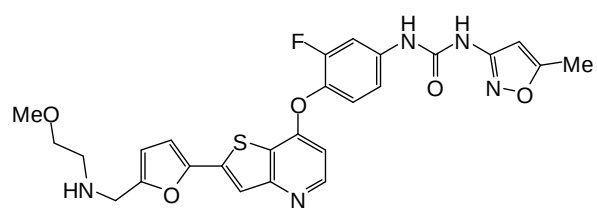
(Cpd. 276, example 169).
