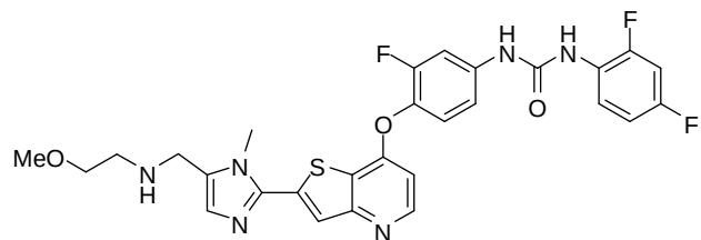
(Cpd. 359 example 245). and
