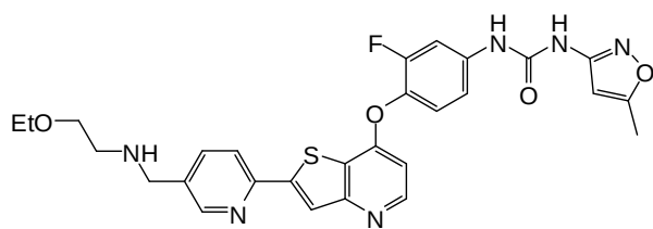
(Cpd. 279, example 172),
