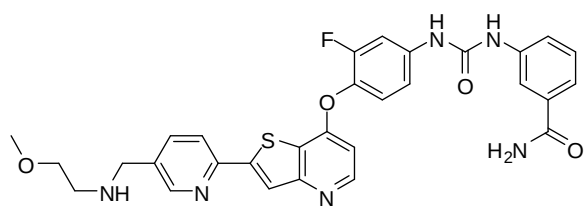
(Cpd. 333, example 219).
