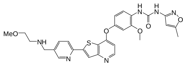
(Cpd. 262, example 155),
