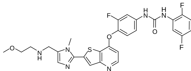
(Cpd. 347 example 233),
