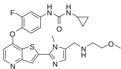
(Cpd. 287, example 179),
