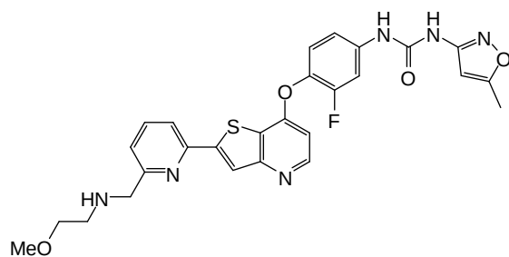
(Cpd. 269, example 162),
