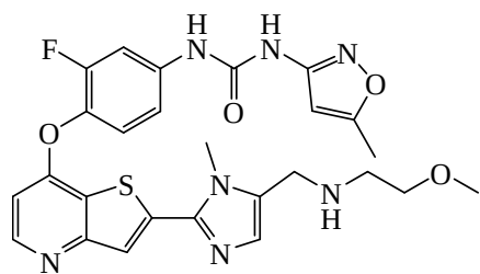
(Cpd. 282, example 175),
