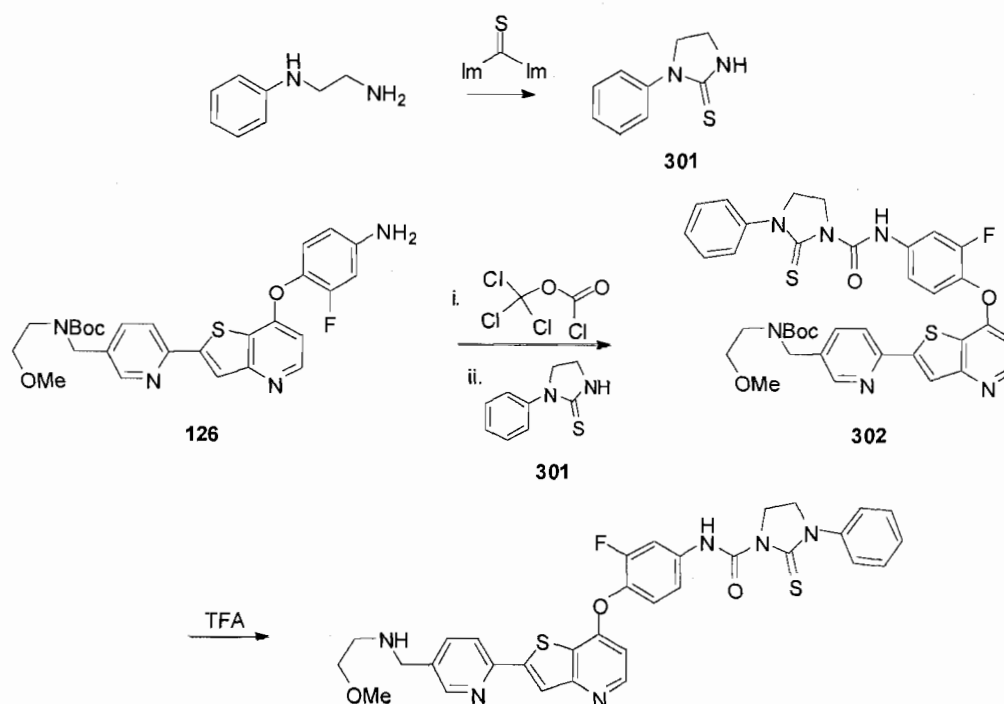
Scheme 16
