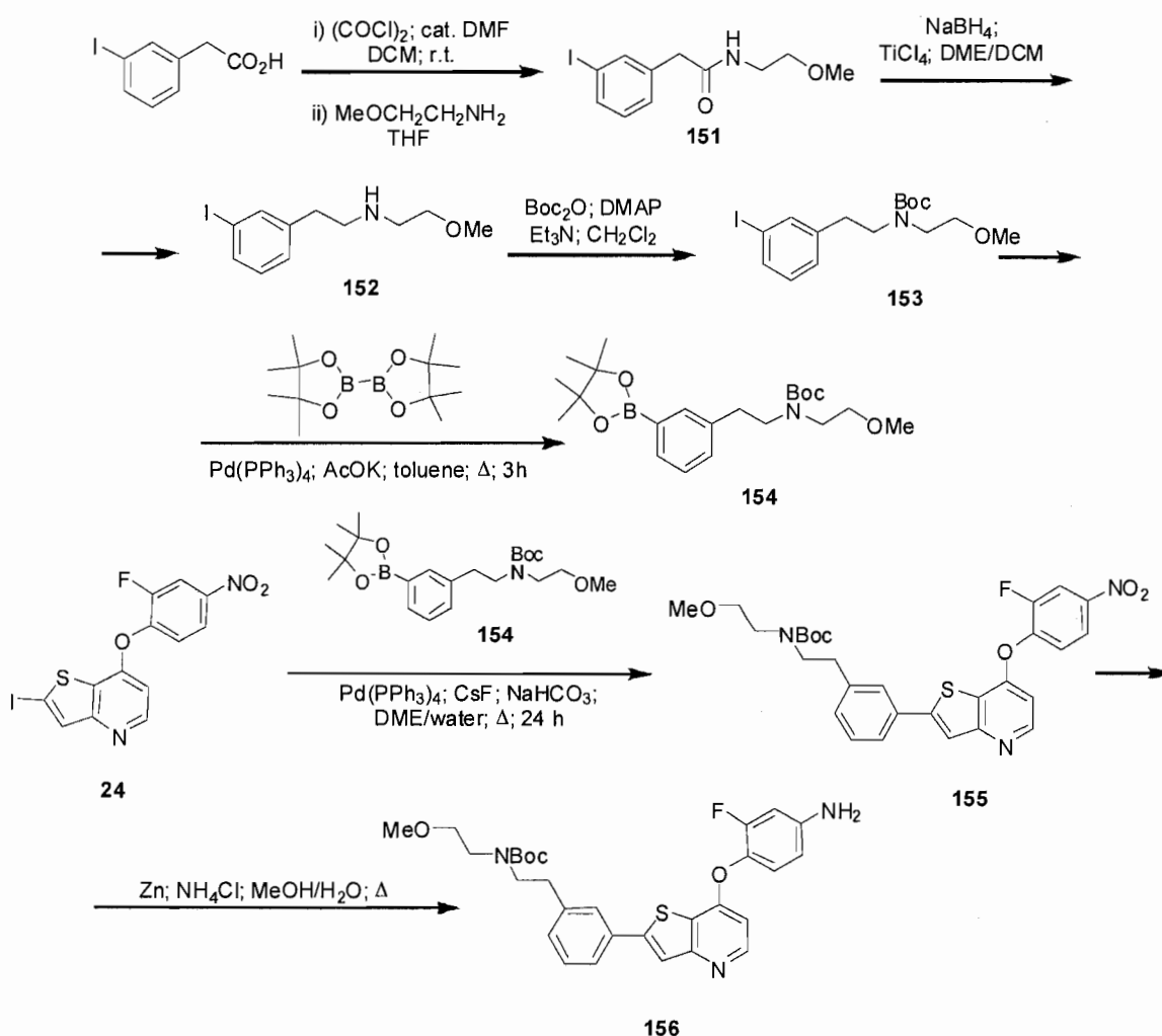
Scheme 12
