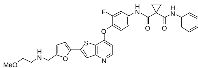
(Cpd. 113, example 39)
