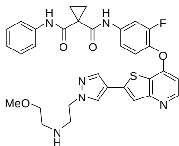
(Cpd. 83, example 26)
