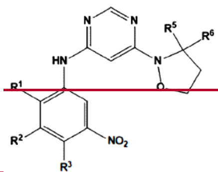
[Chemical Formula 6]
