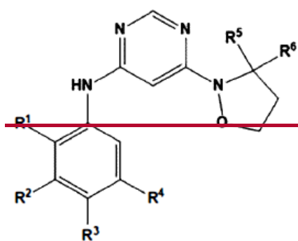
[Chemical Formula 1]
