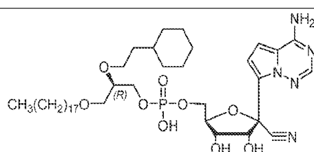
1-O-octadecyl-2-O-(3-cyanobenzyl)- sn -glyceryl-phospho-RVn
