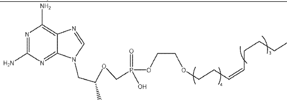
Oleyloxyethyl 9-( R )-[(2-phosphonomethoxy)propyl]-2,6-diaminopurine (OLE-( R )-PMPDAP)
