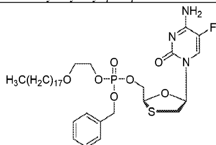
Octadecyloxyethyl benzyl-phospho-emtricitabine (ODE-Bn-P-FTC)
