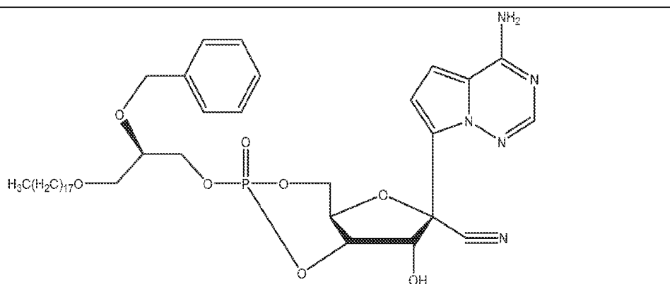
GS-441524-3',5'-cyclic monophosphate, 1-O-octadecyl-2-O-benzyl- sn -glyceryl ester
