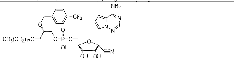
1-O-octadecyl-2-O-(4-trifluoromethyl)- sn -glyceryl- phospho -RVn
