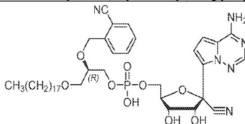
1- O -octadecyl-2- O -(2-cyanobenzyl)- sn -glyceryl- phospho -RVn
