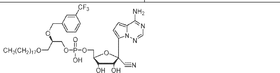
1-O-octadecyl-2-O-(3-trifluoromethyl)- sn -glyceryl- phospho -RVn
