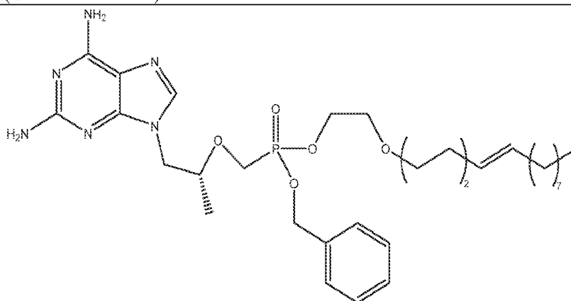
Oleyloxyethyl benzyl 9-( R )-[(2-phosphonomethoxy)propyl]-2,6-diaminopurine (OLE-Bn-PMPDAP)
