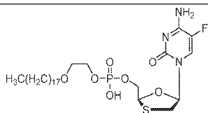
Octadecyloxyethyl- phospho -emtricitabine (ODE-P-FTC)
