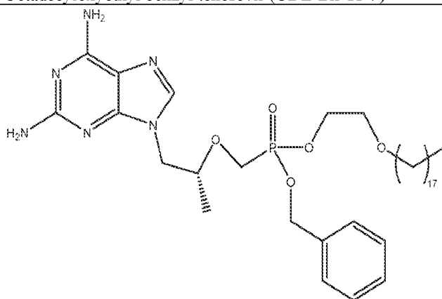
Octadecyloxyethyl benzyl 9-( R )-[(2-phosphonomethoxy)propyl]-2,6-diaminopurine (ODE-Bn-PMPDAP)
