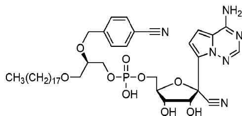
1- O -octadecyl-2- O -(4-cyano)benzyl)- sn -glyceryl-phospho-RVn
