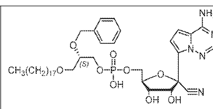
1-O-octadecyl-2-O-(3-cyanobenzyl)- sn -glyceryl-phospho-RVn
