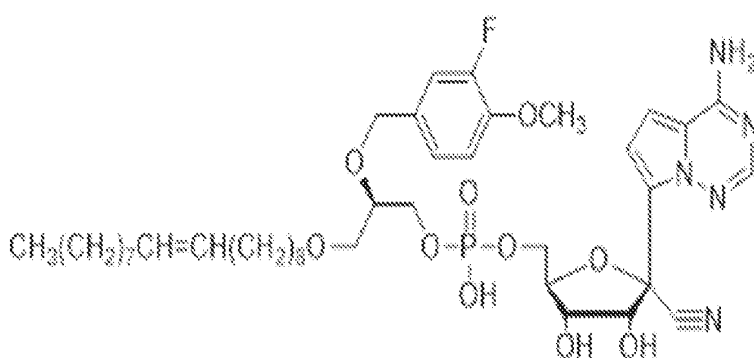
1-O-oleyl-2-O-(3-fluoro, 4-methoxybenzyl)- sn -glyceryl-phospho-RVn
