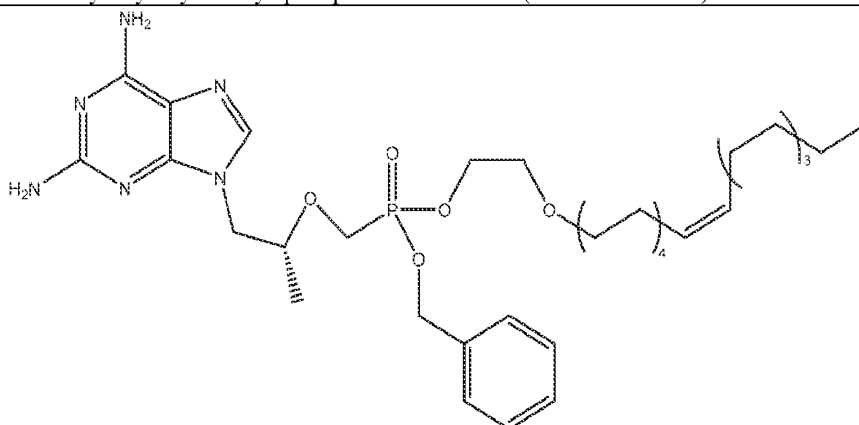
Oleyloxyethyl benzyl 9-( R )-[2-phosphono-methoxy]propyl]-2,6-diaminopurine (OLE-Bn-PMPDAP)
