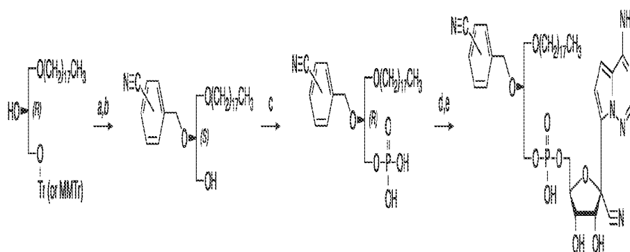
Scheme 7. Synthesis of 2, 3 and 4-cyanobenzyl analogs. Reagents: a) sodium hydride, 2,3 or 4-(bromomethyl)benzonitrile, tetrabutyl ammonium iodide, THF; b) p-TsOH (cat.), CH 2 Cl 2 , MeOH; c) i) POCl 3 , triethylamine, CH 2 Cl 2 , ii) acetone/ice water; d) RVn (GS-441524) acetonide, DIC/NMI, pyridine, 35 °C; e) formic acid, rt.
