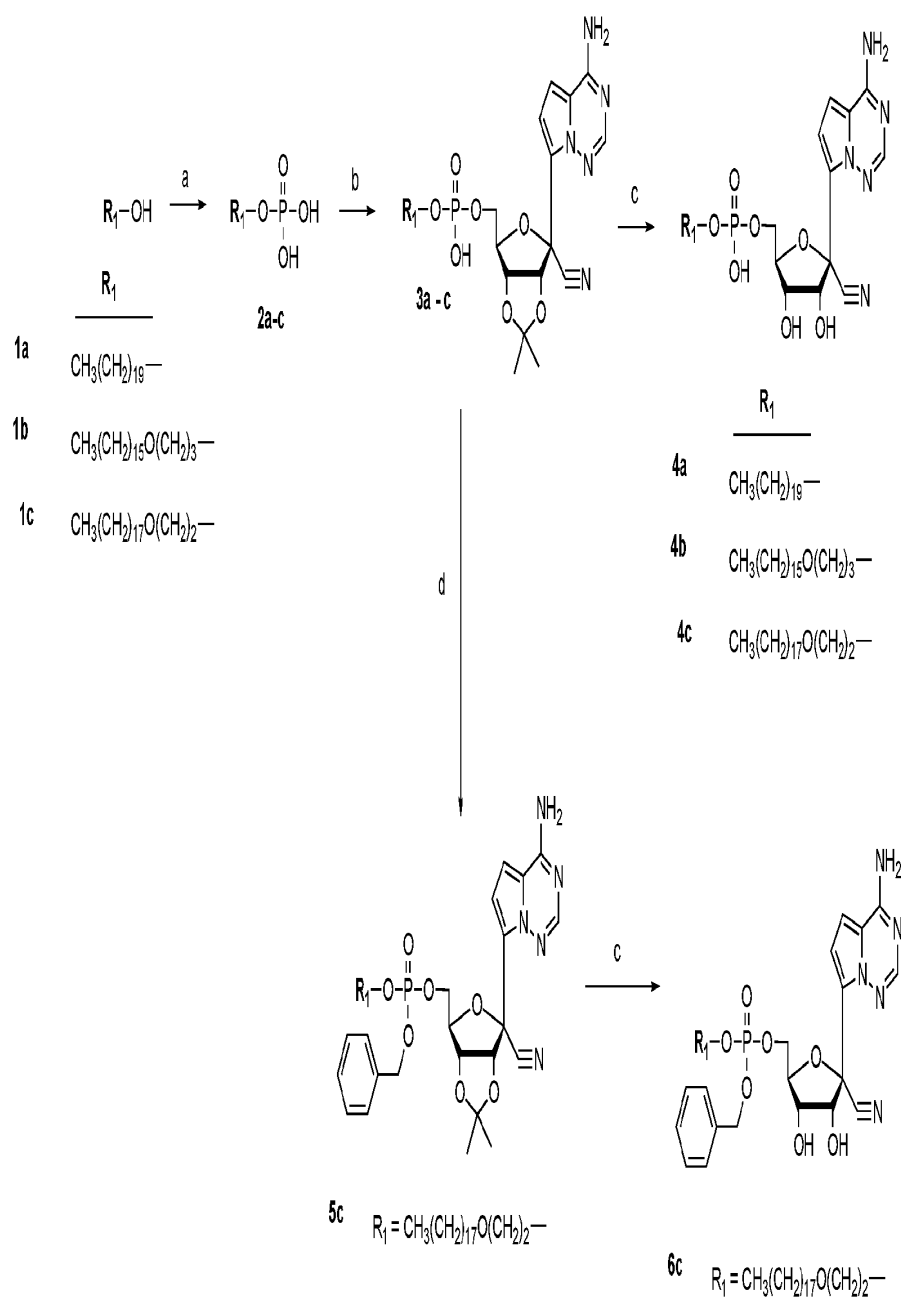
Scheme 1. Synthesis of Alkyl and Alkoxyalkyl Esters of GS-441524 5'-Monophosphate. Reagents: a) POCl 3 , TEA, THF; b) GS-441524 acetonide, DCC/DMAP or DIC/NMI, pyridine; c) formic acid, rt or con. HCl/THF; d) Py BOP, DIEA, DMF
