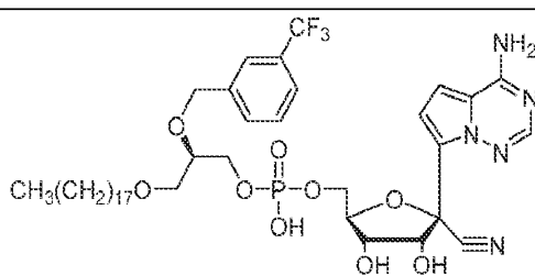
1- O -octadecyl-2- O -(3-trifluoromethyl)- sn -glyceryl- phospho -RVn
