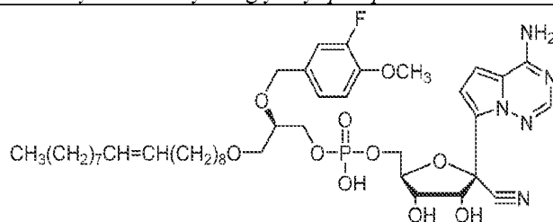
1- O -oleyl-2- O -(3-fluoro, 4-methoxybenzyl)- sn -glyceryl- phospho -RVn
