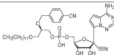
1-O-octadecyl-2-O-(4-cyano)- sn -glyceryl-phospho-RVn
