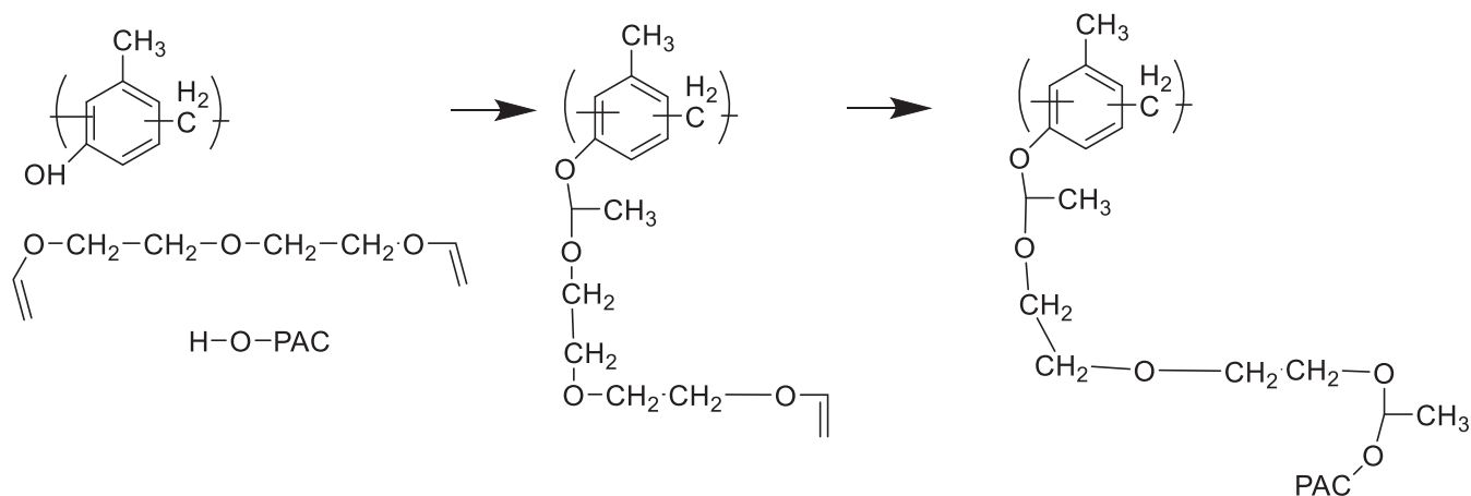
Scheme 5
