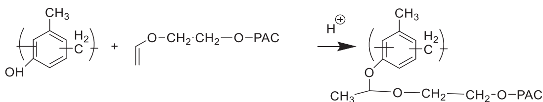
Scheme 10
