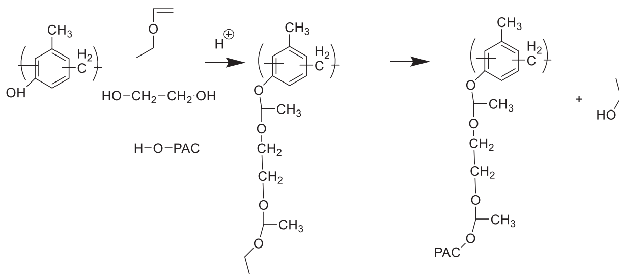
Scheme 7
