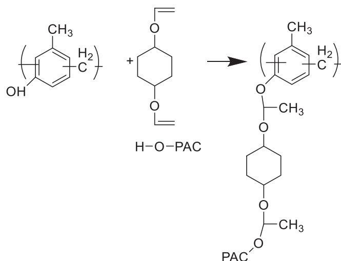
Scheme 5
