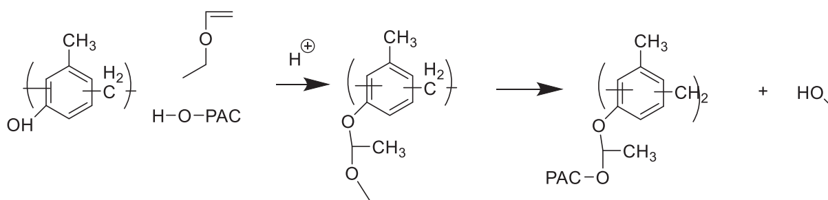
Scheme 9
