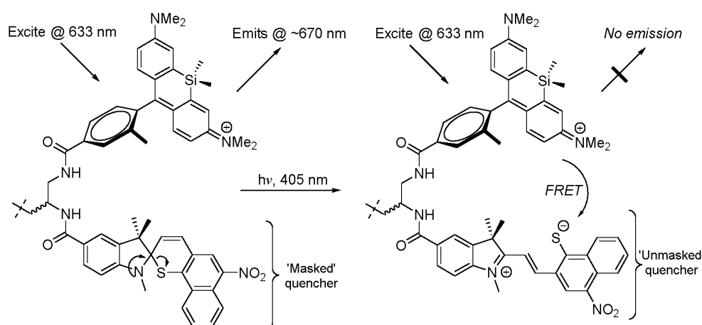
Scheme 1. Photochemical quenching of dyad with silicon-containing rhodamine fluorescent moiety.
