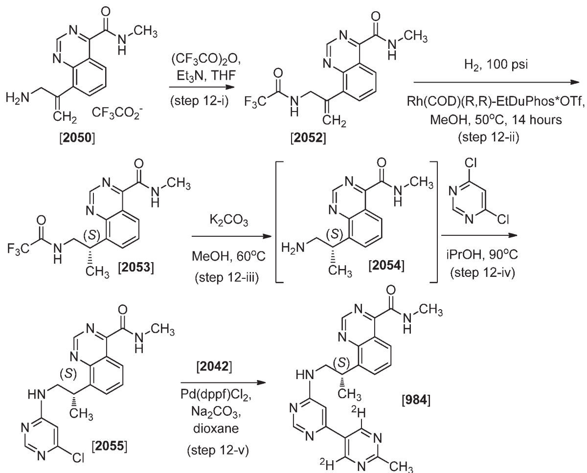
Scheme 12
