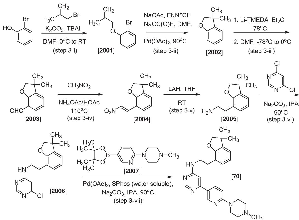
Scheme 3
