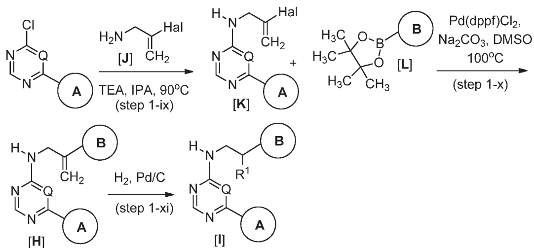
Scheme 1 – Method D
