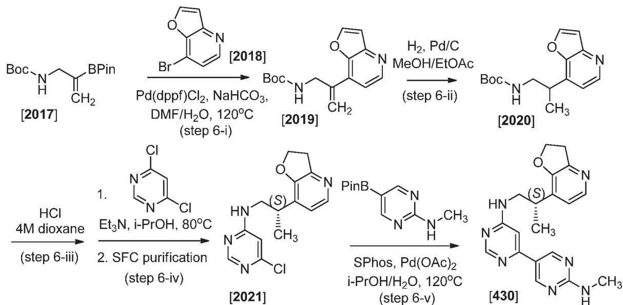
Scheme 6
