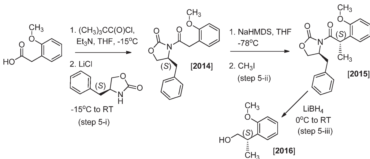
Scheme 5
