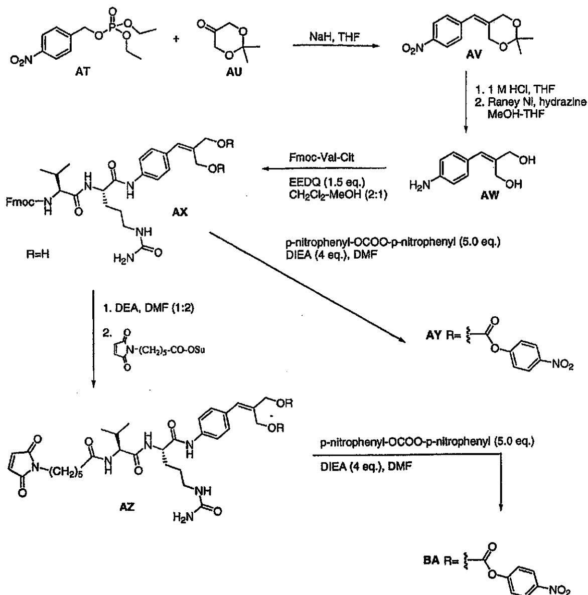
Scheme 15
