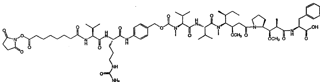
Compound 17
