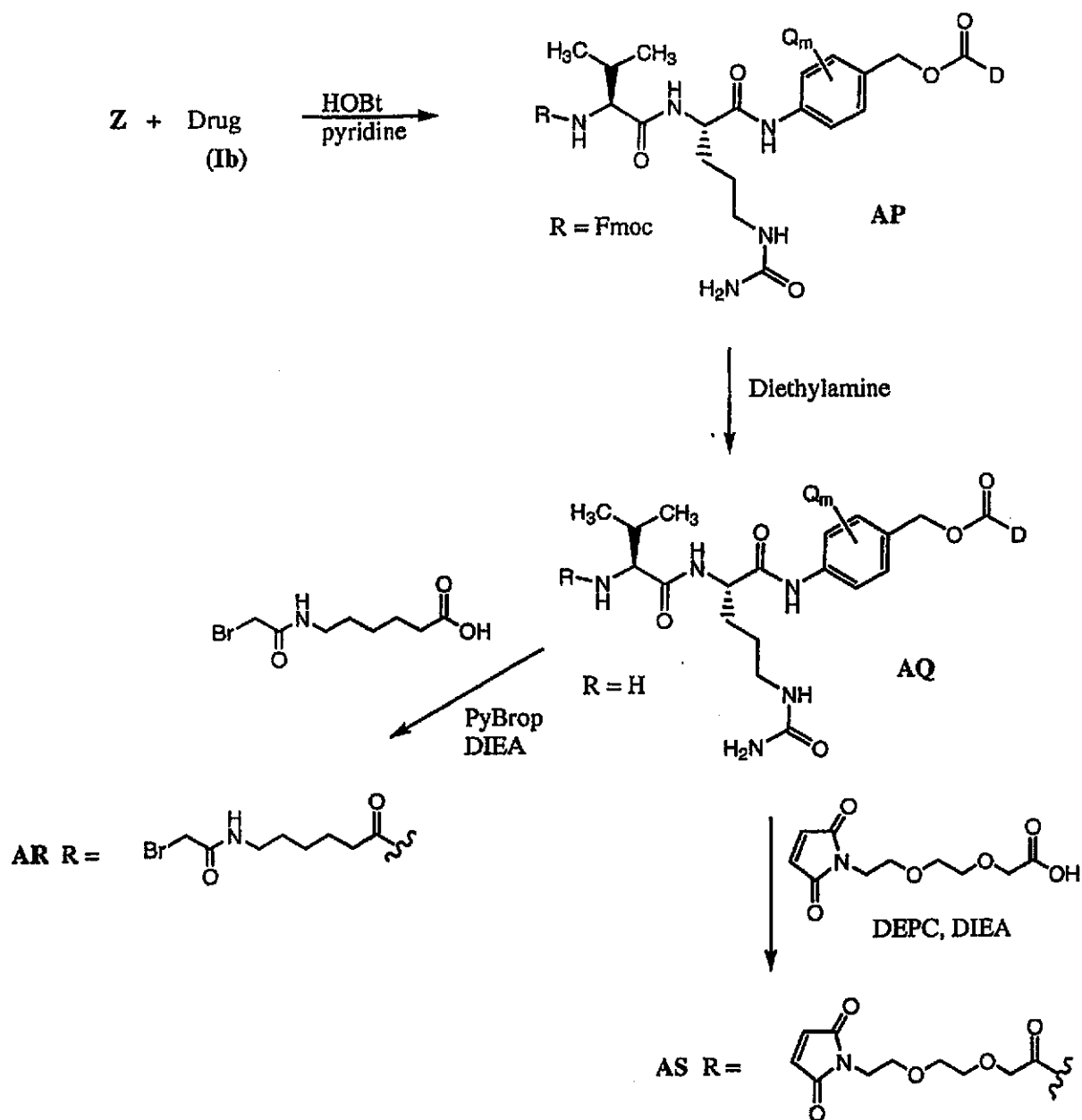
Scheme 14
