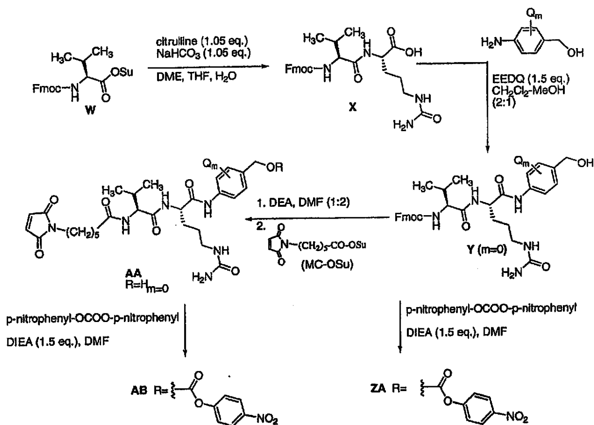
Scheme 11
