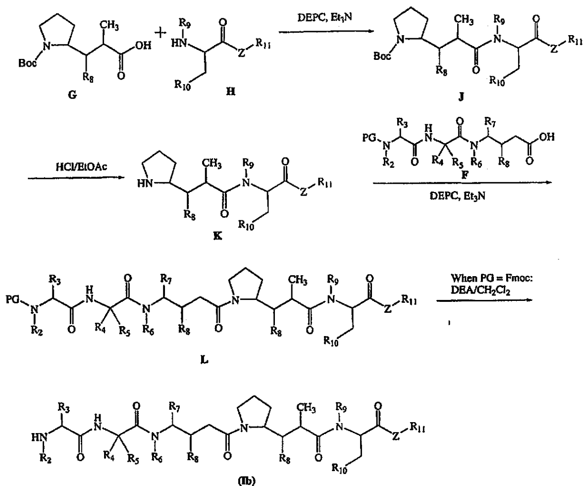
Scheme 6
