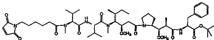
MC-MeVal-Val-Dil-Dap-Phe-OtBu
