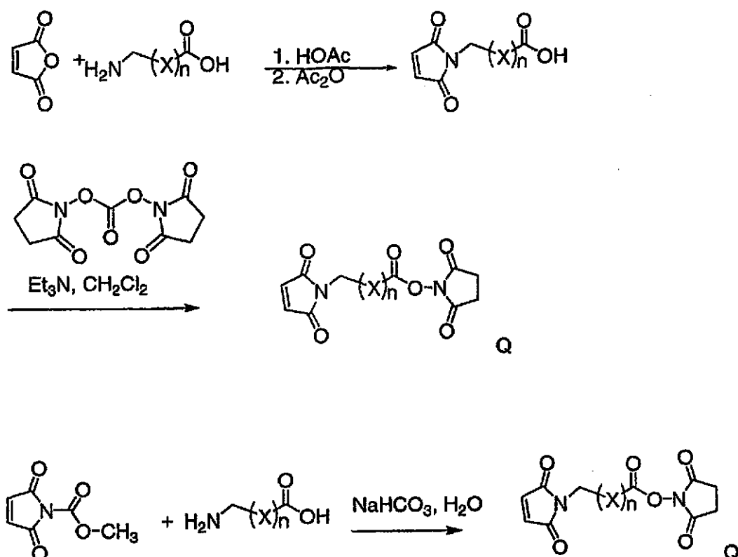
Scheme 8
