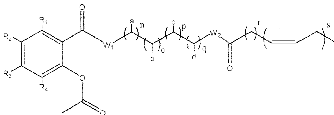
Formula 1c'
