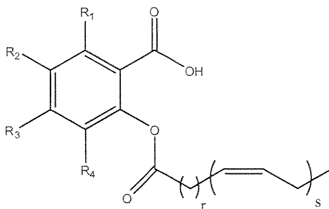
Formula Ia
