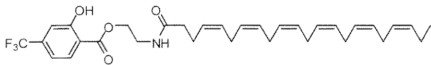
VIc-1
