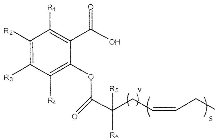
Formula Ia'
