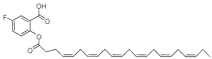
Ia-5
