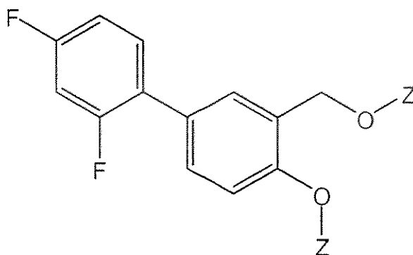
Formula IVd
