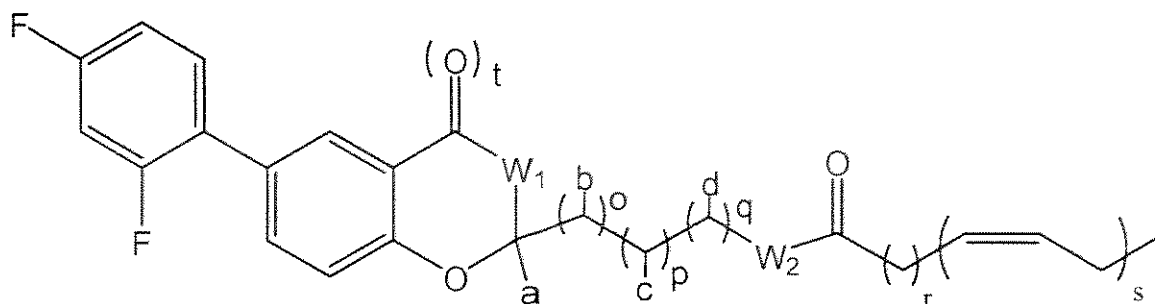
Formula IVe
