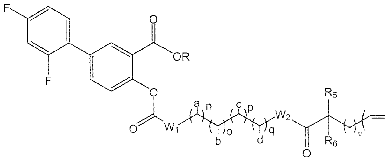
Formula IVg'
