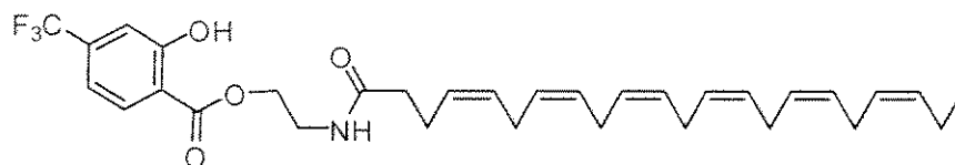
VIc-4
