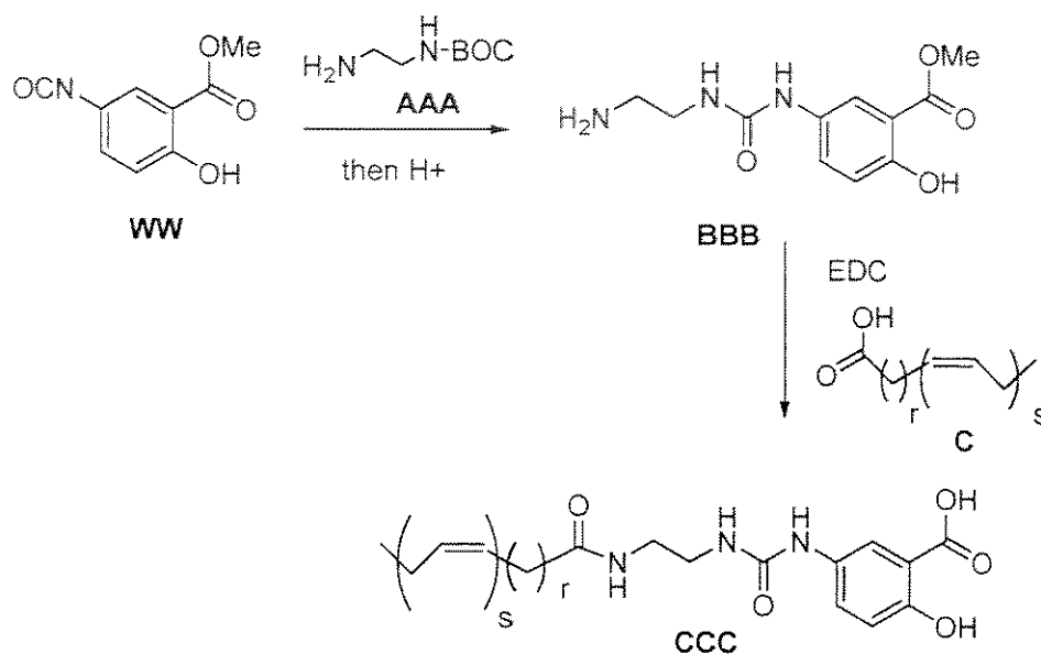
Scheme 17
