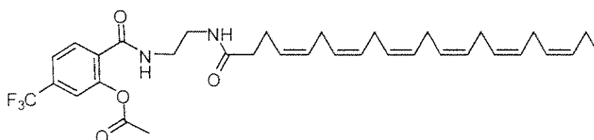
VIb-12
