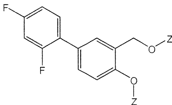
Formula IVd'
