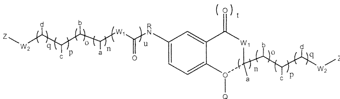
Formula III
