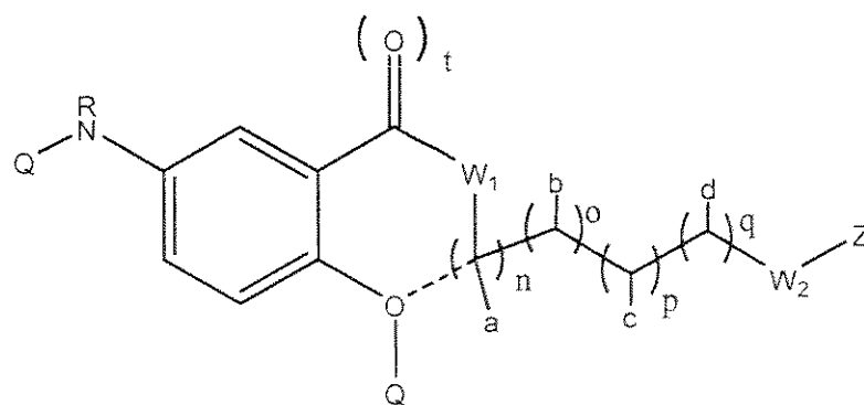
Formula IIIa'
