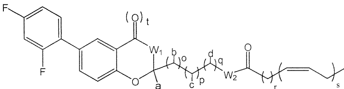
Formula IVe
