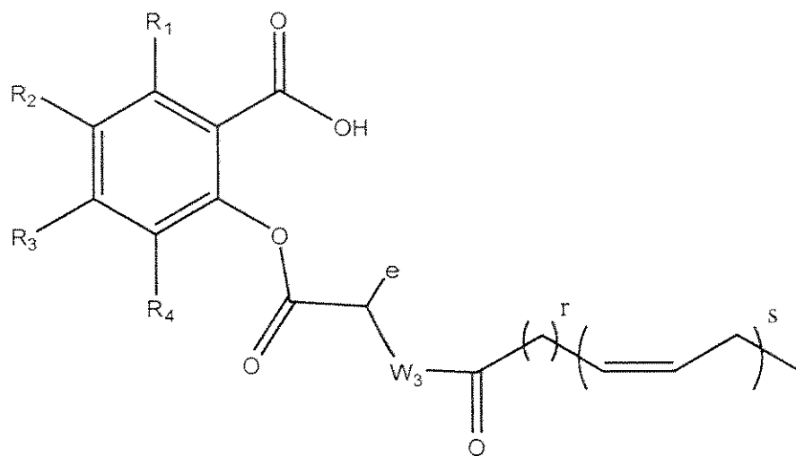
Formula Ig
