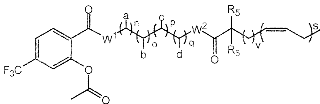
Formula Vlb'
