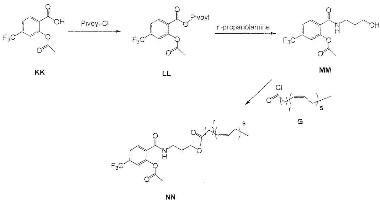
Scheme 12
