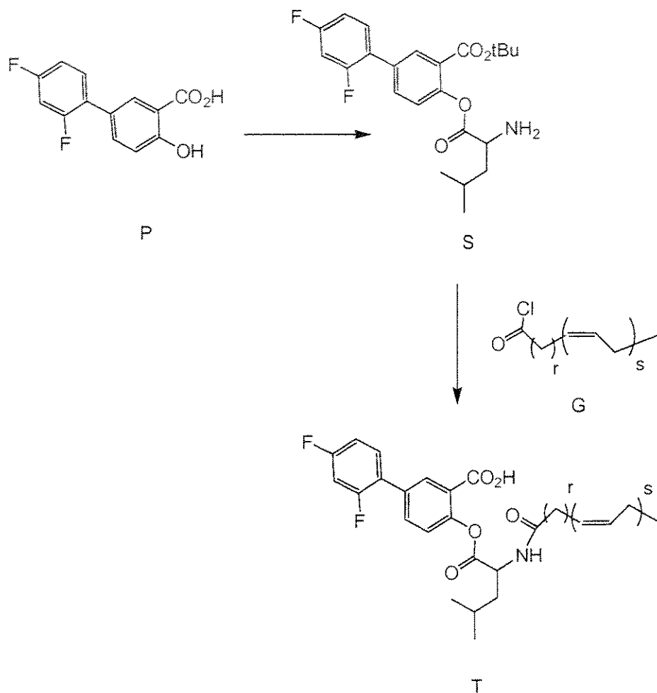
Scheme 6
