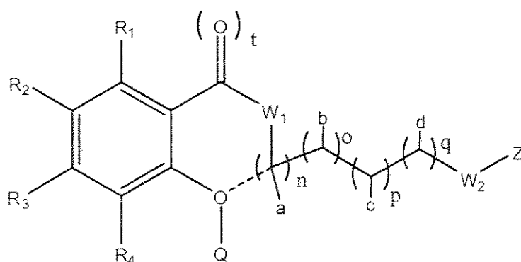
Formula II
