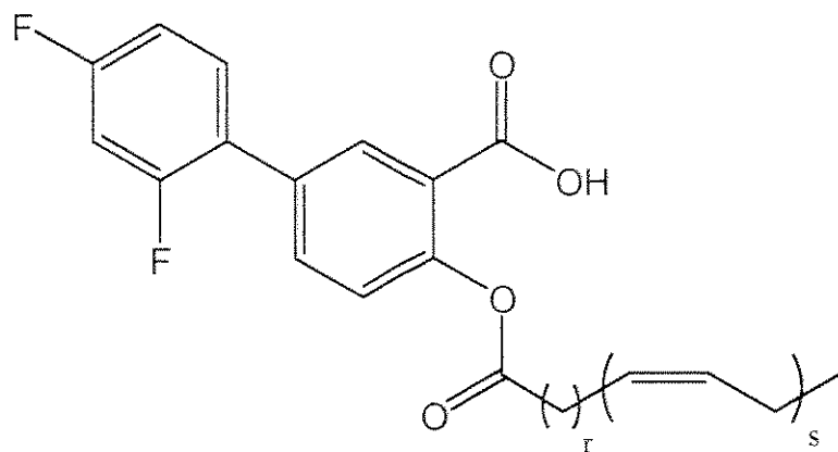
Formula IVa
