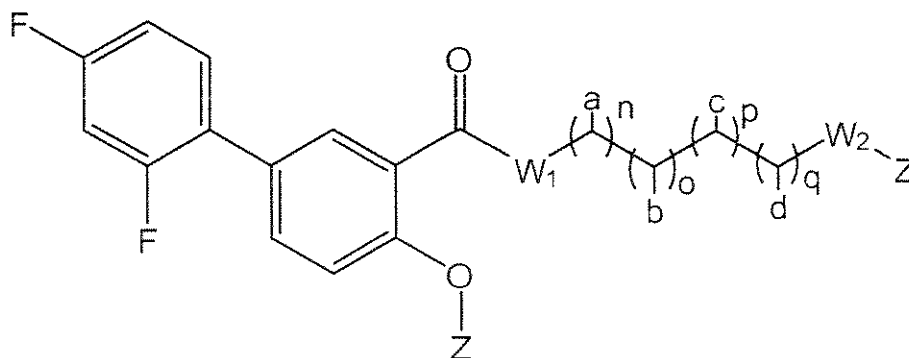
Formula IVc'
