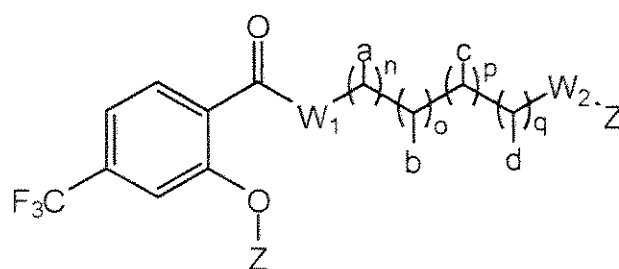
Formula VIc
