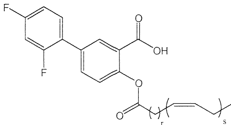
Formula IVa
