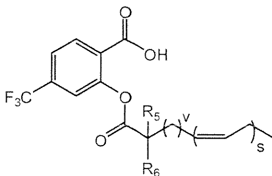
Formula VIa'
