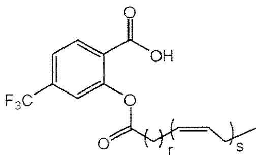
Formula VIa
