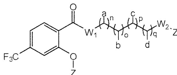
Formula VIc
