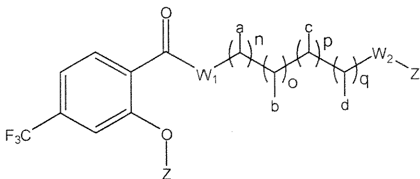
Formula VIc'
