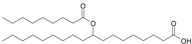
[Chem 13]
