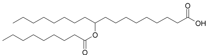
[Chem 13]
