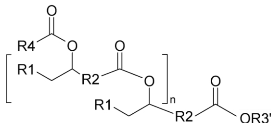
[Chem 10]:
