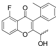
Intermediate 153
