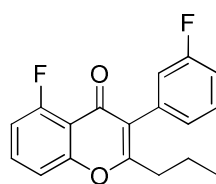
Intermediate 136
