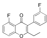
Intermediate 21
