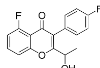
Intermediate 109
