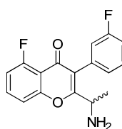
Intermediate 143
