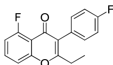
Intermediate 30
