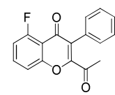
Intermediate 112
