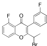
Intermediate 22
