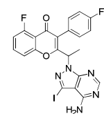
Intermediate 34
