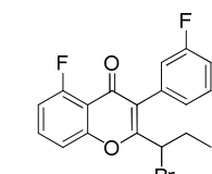
Intermediate 137
