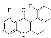
Intermediate 133
