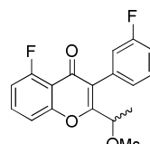
Intermediate 141
