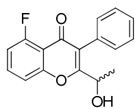
Intermediate 116
