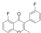
Intermediate 16
