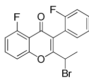
Intermediate 134
