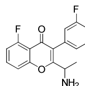
Intermediate 36
