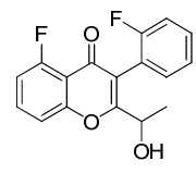
Intermediate 135
