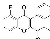
Intermediate 91
