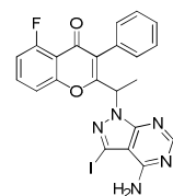
Intermediate 108
