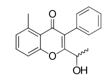
Intermediate 149
