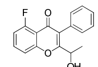
Intermediate 110
