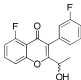
Intermediate 26
