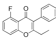
Intermediate 32
