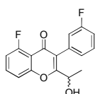
Intermediate 25
