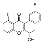
Intermediate 23
