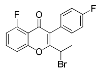
Intermediate 31
