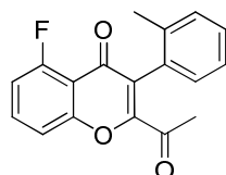
Intermediate 152
