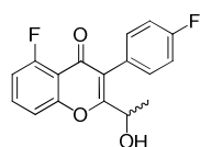
Intermediate 114
