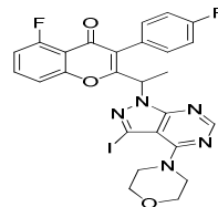
Intermediate 105
