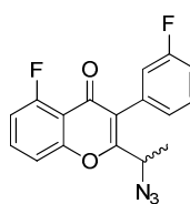
Intermediate 142
