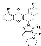
Intermediate 106
