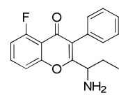
Intermediate 93
