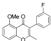
Intermediate 9
