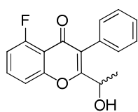
Intermediate 115
