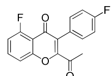
Intermediate 111
