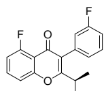
Intermediate 23b
