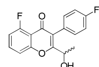
Intermediate 113
