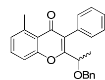
Intermediate 148
