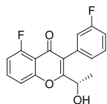
Intermediate 23a
