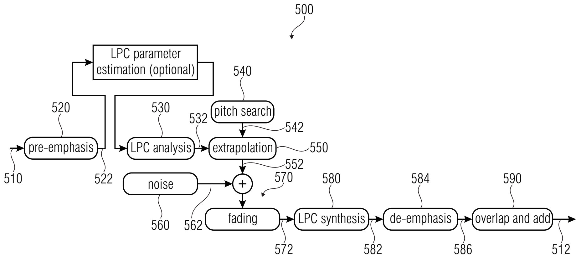
Time domain concealment overview for transform decoder FIG 5
