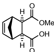
a) (1 S ,2 S ,3 R ,4 R )-3-(Methoxycarbonyl)bicyclo[2.2.1]hept-5-ene-2-carboxylic acid
