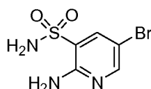
a) 2-Amino-5-bromo-pyridine-3-sulfonic acid amide
