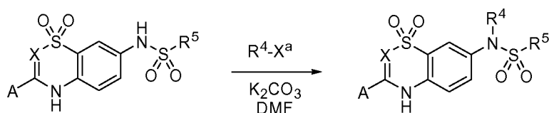
Scheme 26
