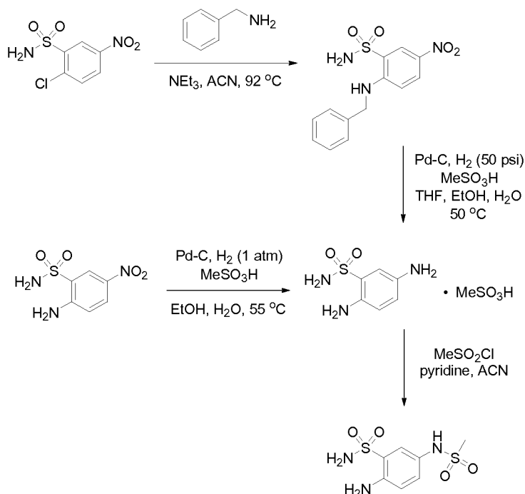
Scheme 16
