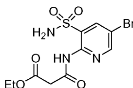
b) N -(5-Bromo-3-sulfamoyl-pyridin-2-yl)-malonamic acid ethyl ester
