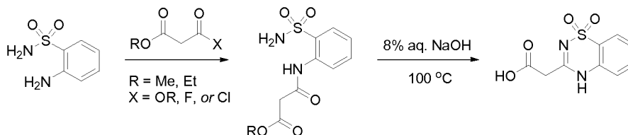
Scheme 18
