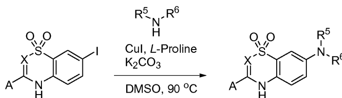
Scheme 28
