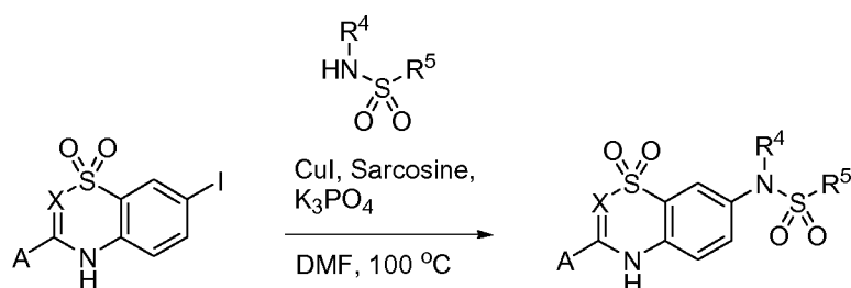
Scheme 24
