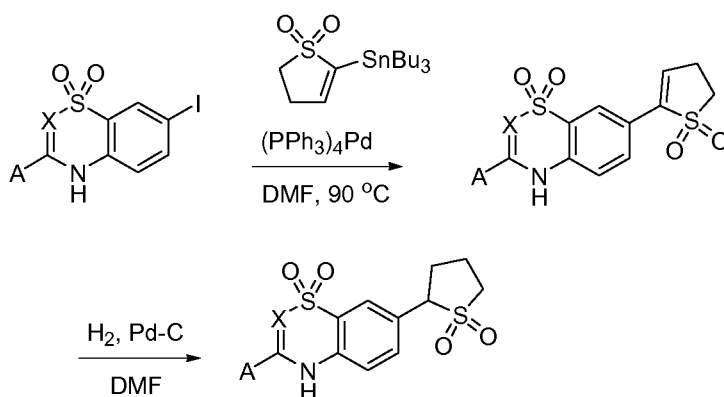
Scheme 27
