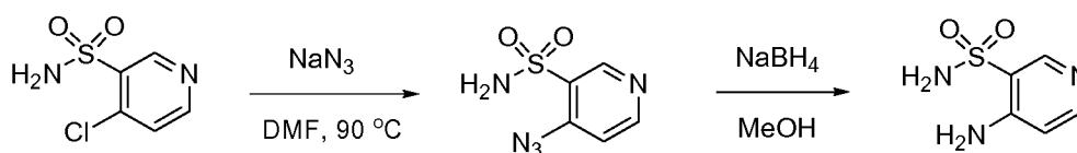
Scheme 22
