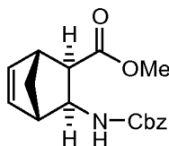
b) Methyl (1 R ,2 R ,3 S ,4 S )-3-[(benzyloxy)carbonyl]amino} bicyclo[2.2.1]hept-5-ene-2-carboxylate
