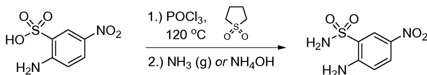
Scheme 15
