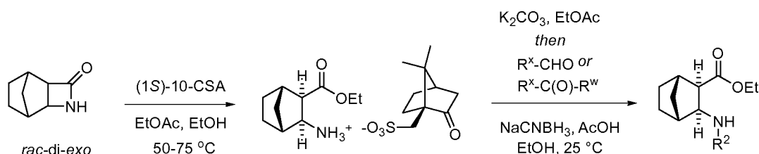
Scheme 8
