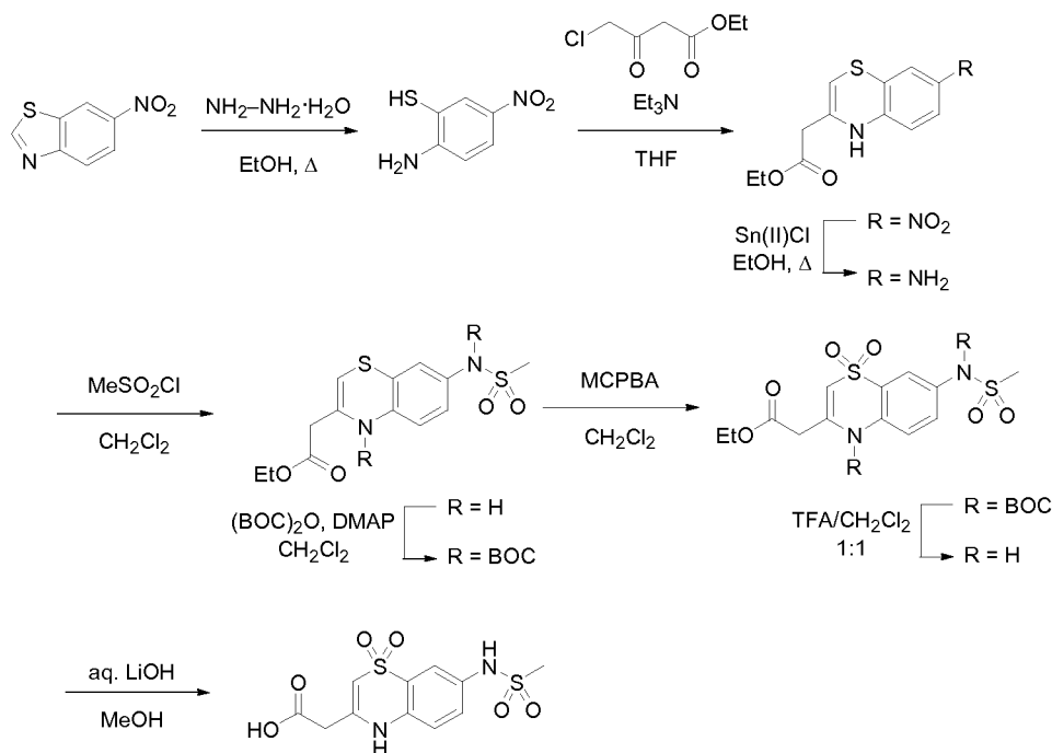
Scheme 13
