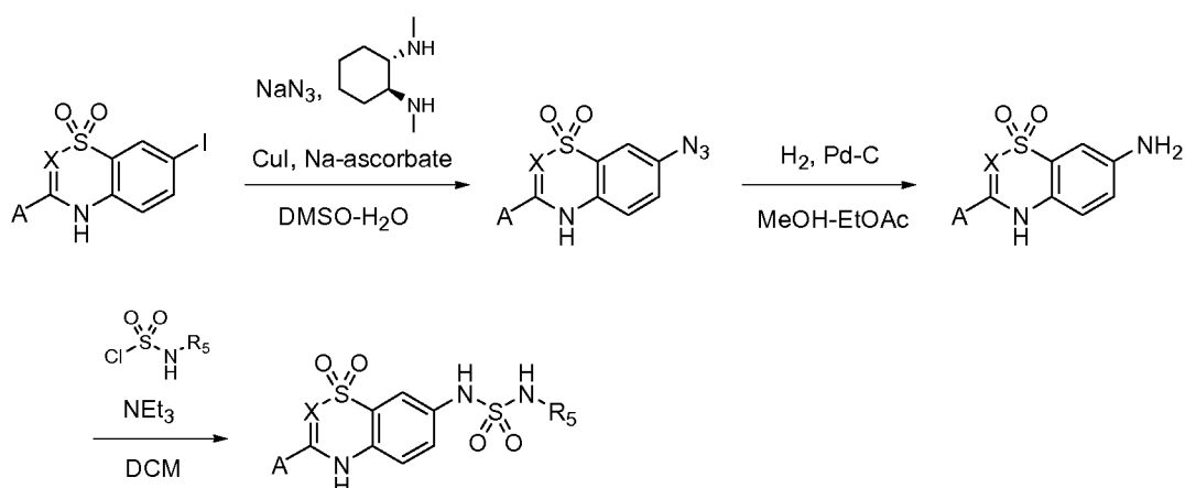
Scheme 25
