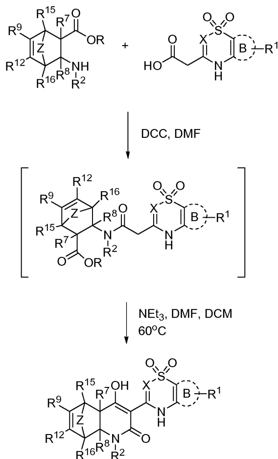
Scheme 2
