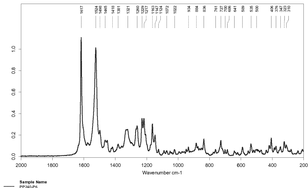
Graph 2. FT-Raman Spectrum.
