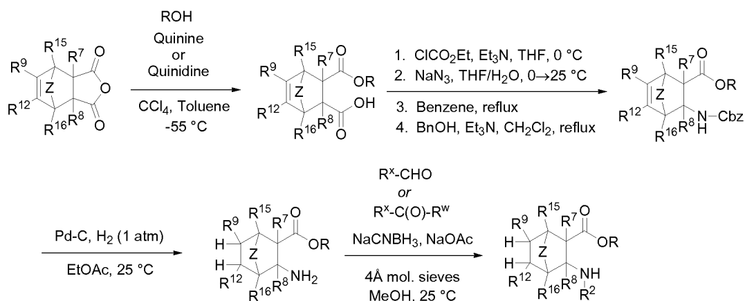
Scheme 4
