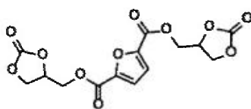
bis((2-oxo-1,3-dioxolan-4-yl)methyl)furan-2,5-dicarboxylate ( FBC-1 );
