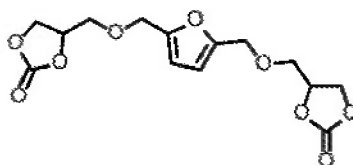
25 4,4'-(((furan-2,5-diylbis(methylene))bis(oxy))bis(methylene))bis(1,3-dioxolan-2-one) ( FBC-2 );
