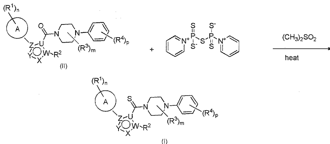
Reaction Scheme 1
