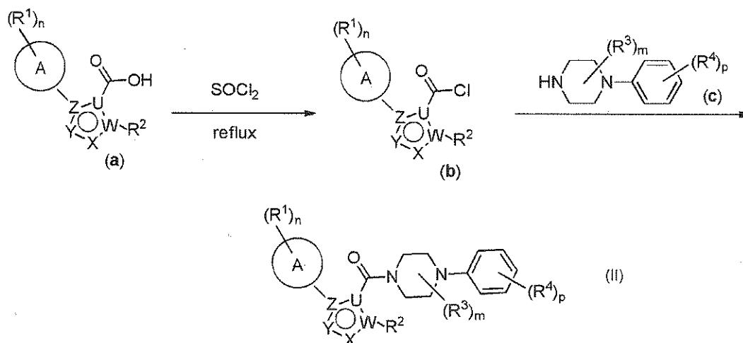
Reaction Scheme 2
