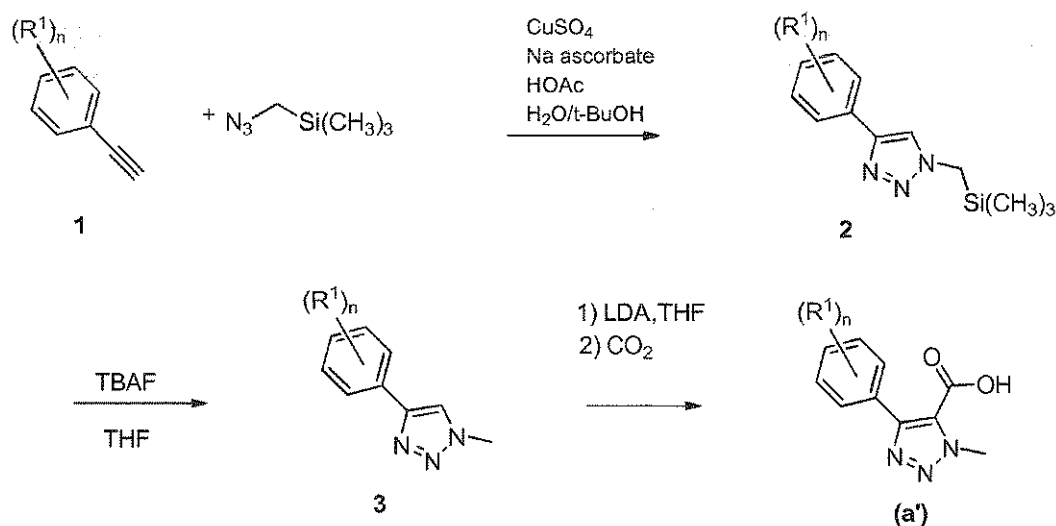
Reaction Scheme 3
