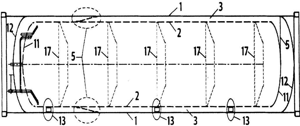
FIG. 1 - state of art vessel
