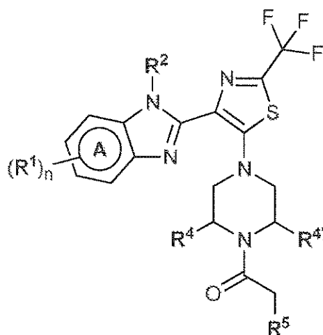
Formula (II)
