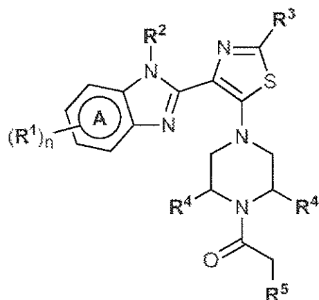
Formula (III)
