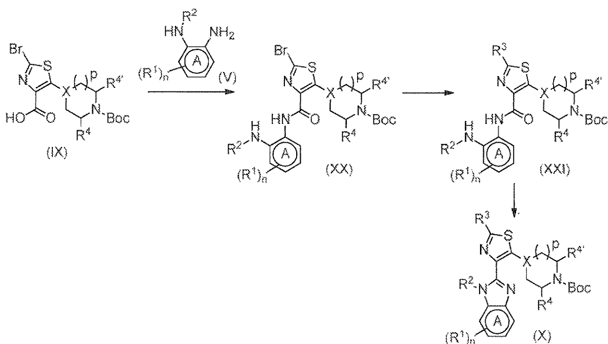
Scheme 14
