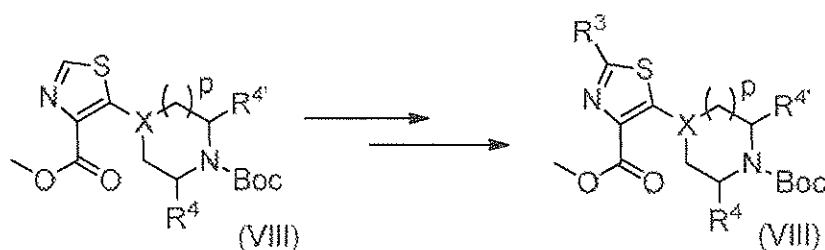
Scheme 10
