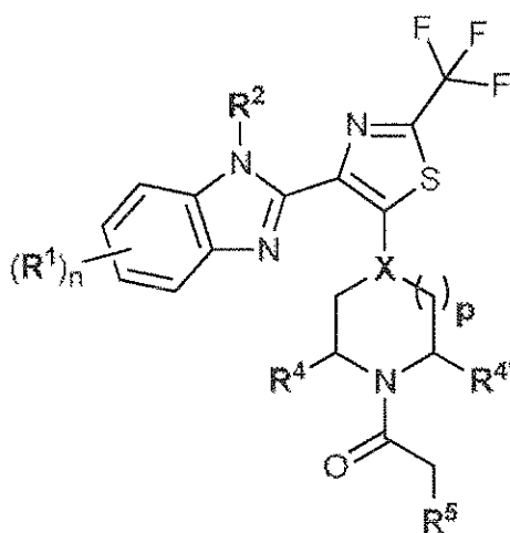
Formula (V)
