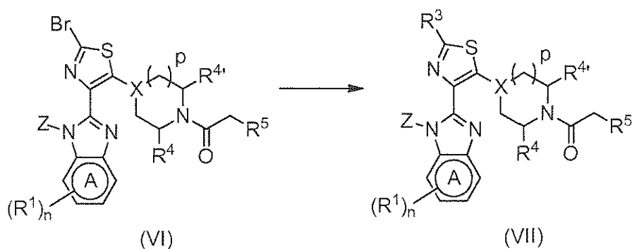
Scheme 4
