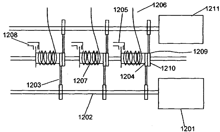
FIGURE -12 VIEW OF MULTIPLE CABLE SPOOL DRIVE
