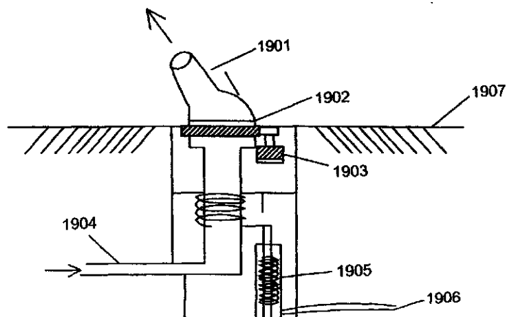
FIGURE 19 COLD AIR NOZZLE WITH ROTATION DRIVE MOTOR AND RETRACTION SOLENOID
