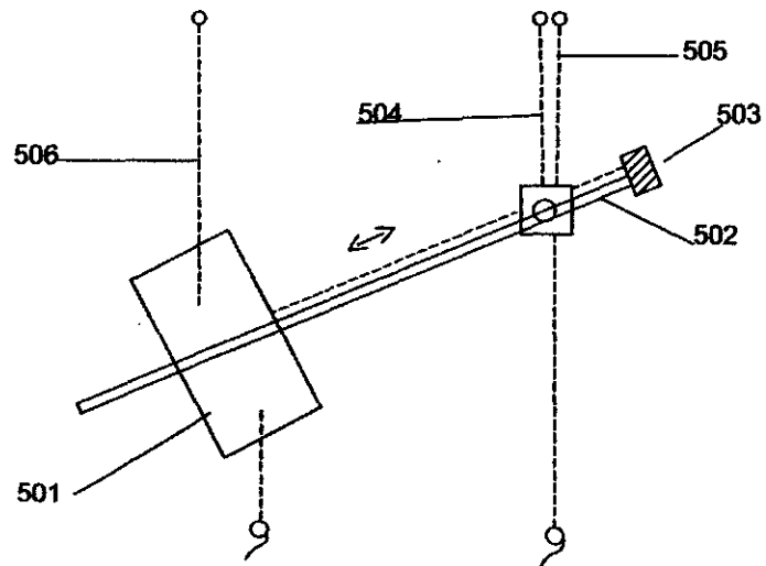
FIGURE - 5 SHADING UNIT WITH CANTILEVER ARM
