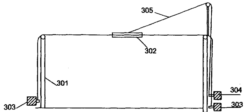
FIGURE - 3 CROSS SECTION VIEW OF SHADING UNIT DRIVE AND POSITIONER
