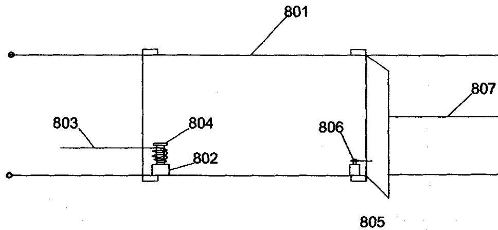
FIGURE:8 SHADDING UNIT WITH ON BOARD MOTOR DRIVE
