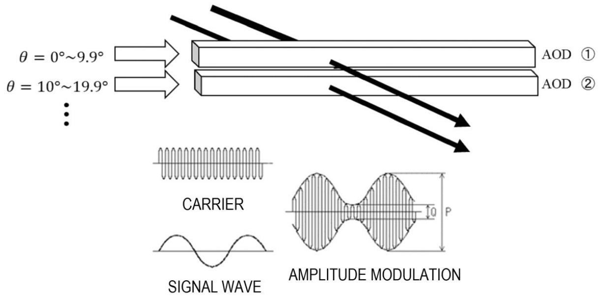
AOD-DRIVEN SIGNAL WAVE
