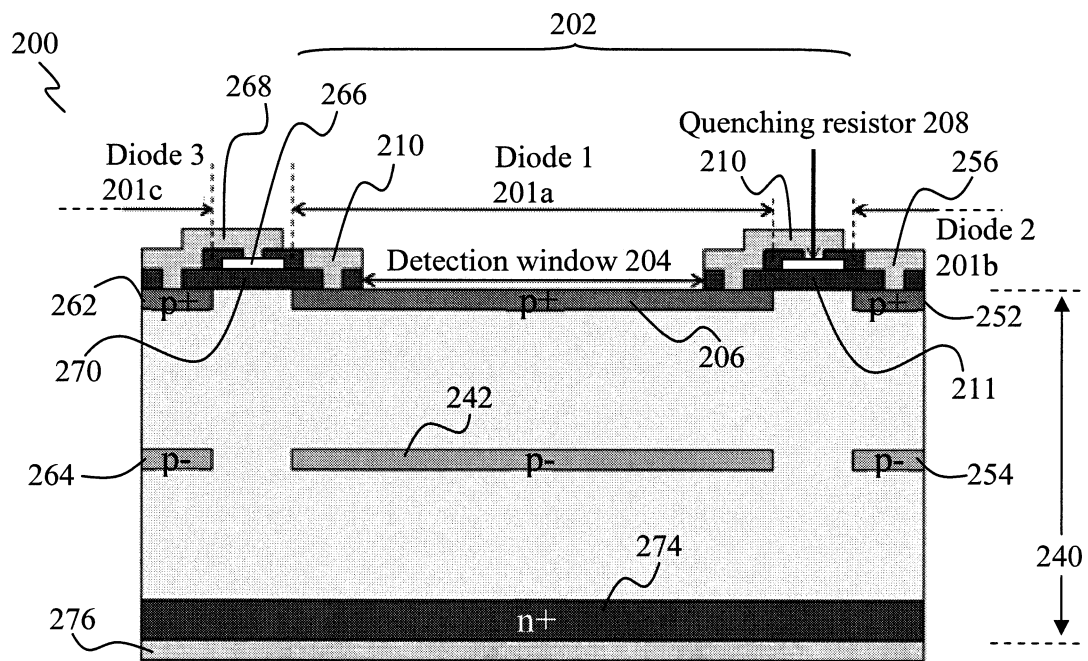
FIG. 2B (CONVENTIONAL)
