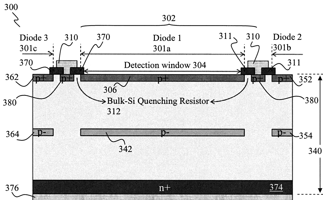
FIG. 3 (PRIOR ART)
