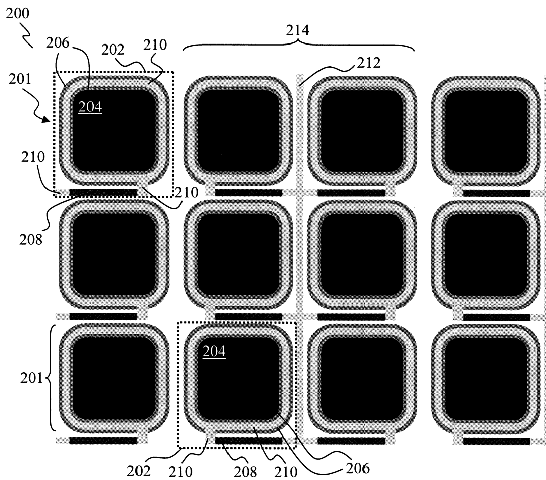
FIG. 2A (CONVENTIONAL)
