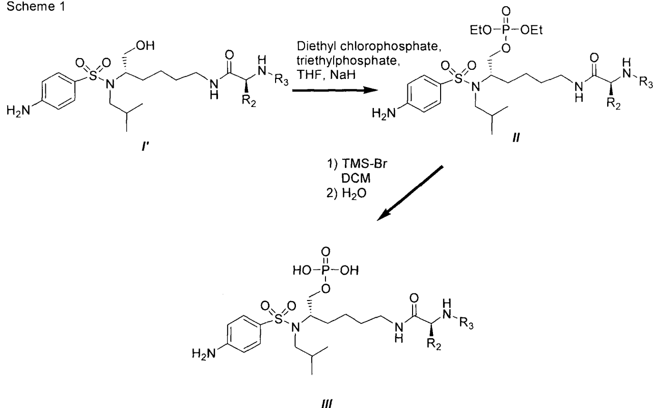
Scheme 1
