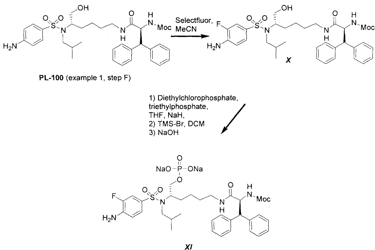
Scheme 3
