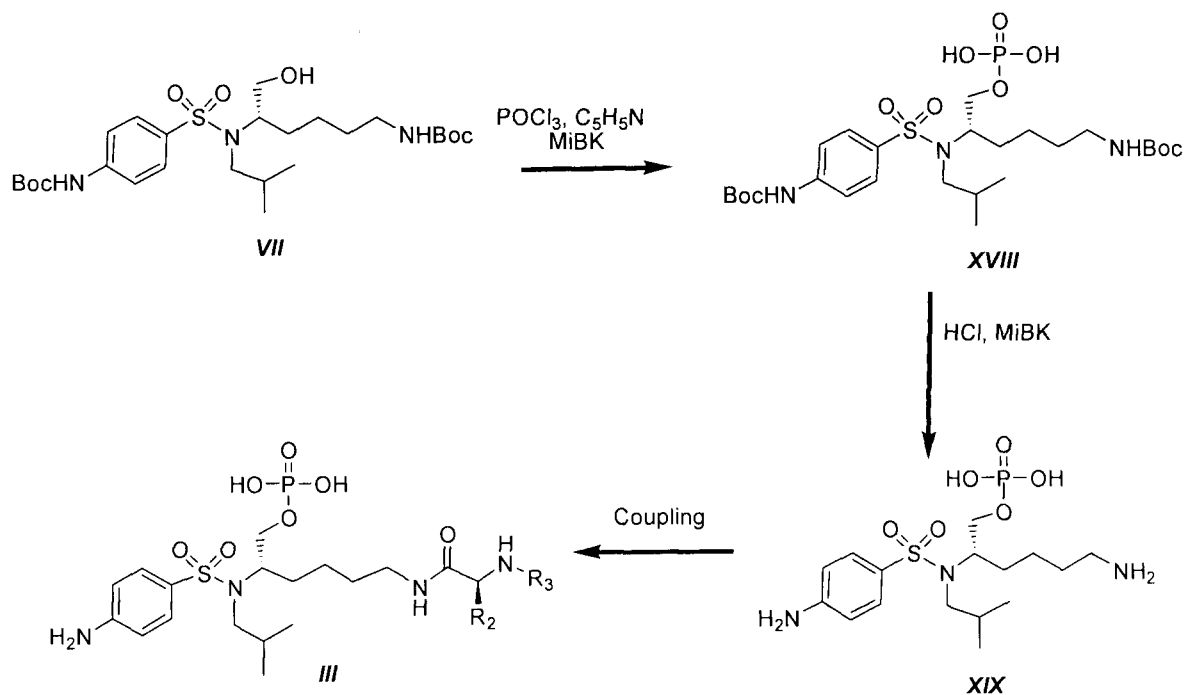
Scheme 2B
