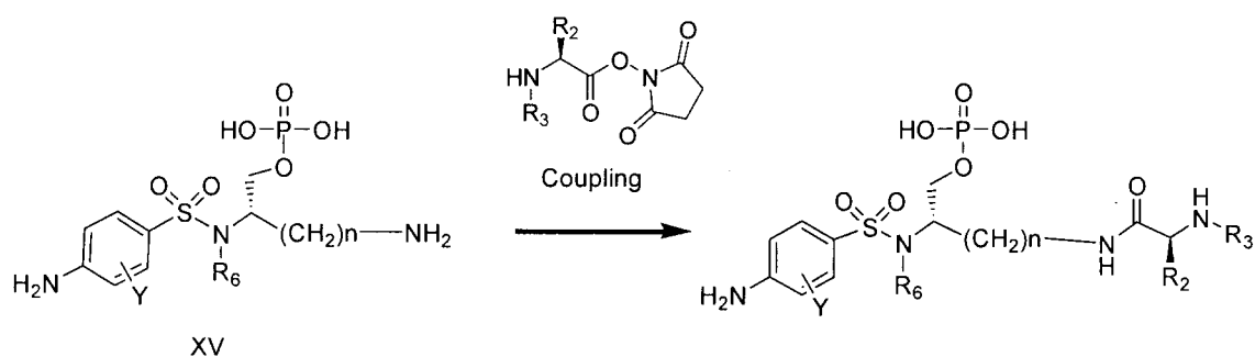
Scheme 2D
