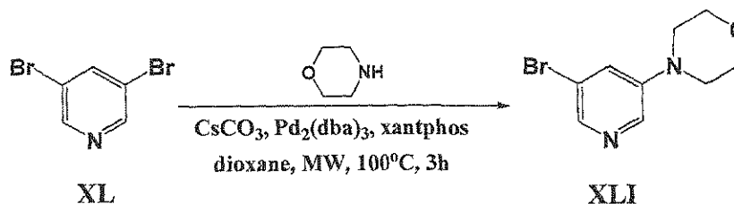
Scheme 7
