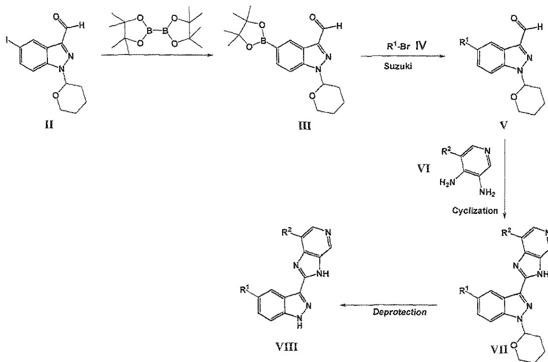
Scheme 1
