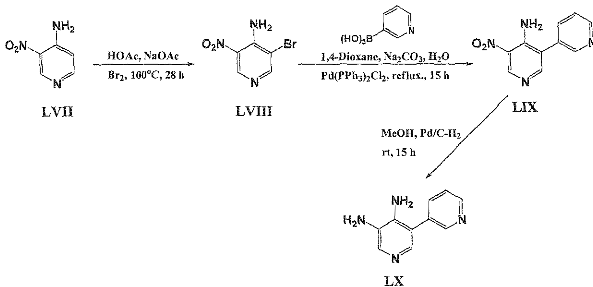
Scheme 12
