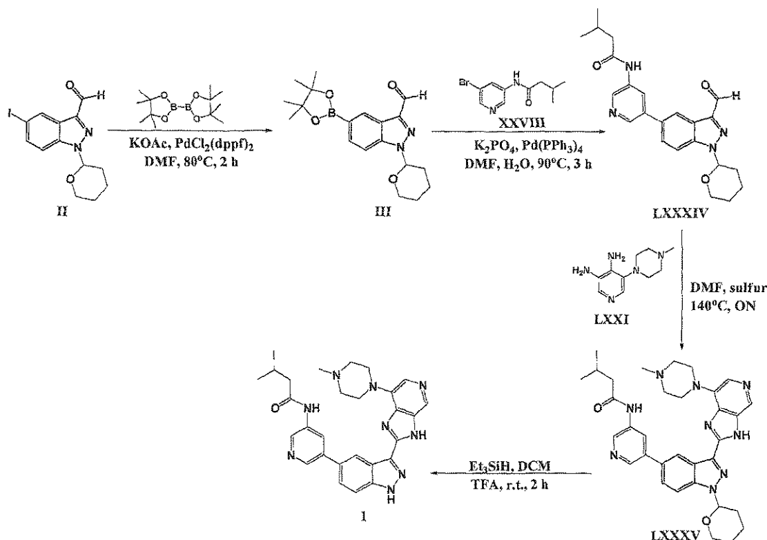
Scheme 16
