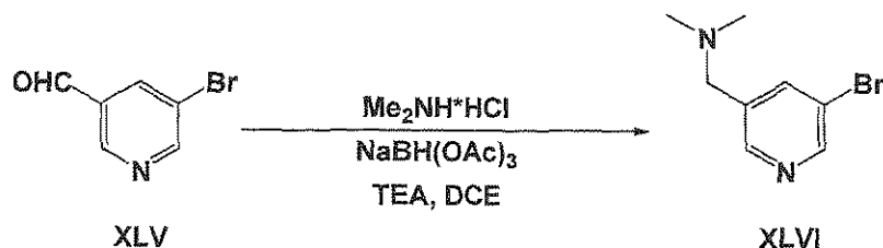
Scheme 10
