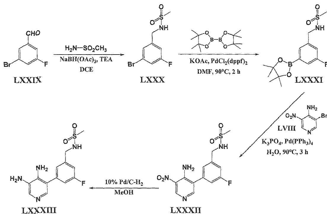
Scheme 15
