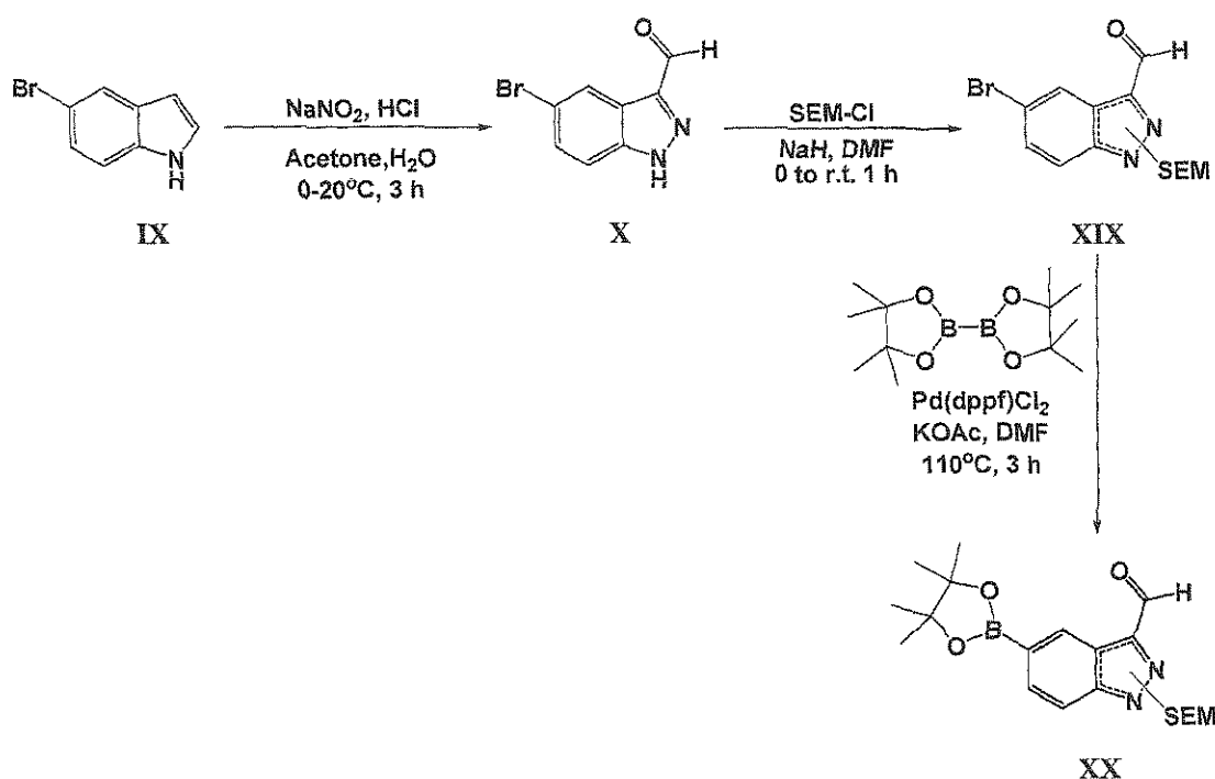
Scheme 4
