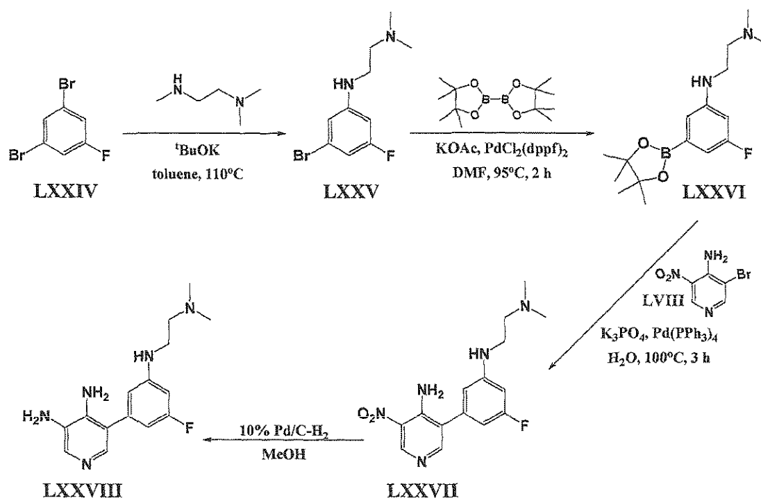
Scheme 14
