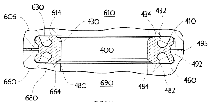
DETAIL B Fig. 6B
