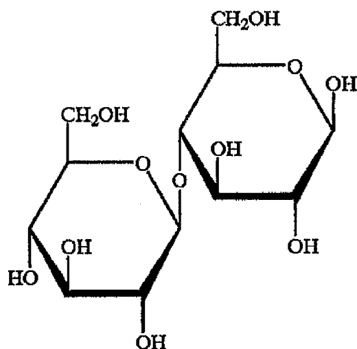
Cellobiose (4-O- \beta -D-Glucopyranosyl-D-glucose)
