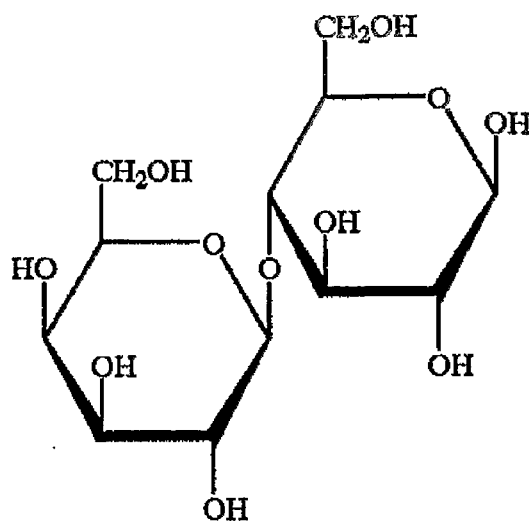
Lactose (4-O- \beta -D-Galactopyranosyl-D-glucose)
