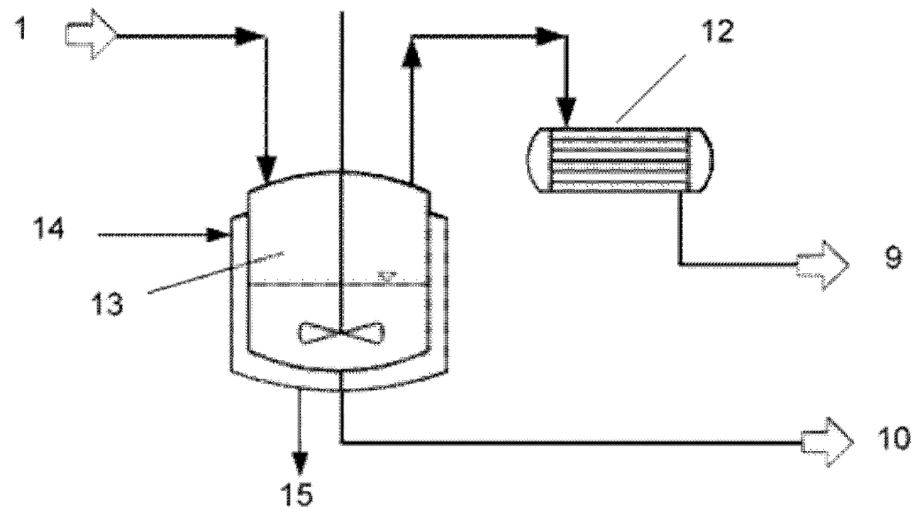
Figure 3: Discontinuous process for obtaining 2-EHA.
