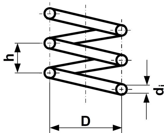
Fig. 1: Sketch of the geometry of a helical tube (5) in a helical-tube evaporator (4).
