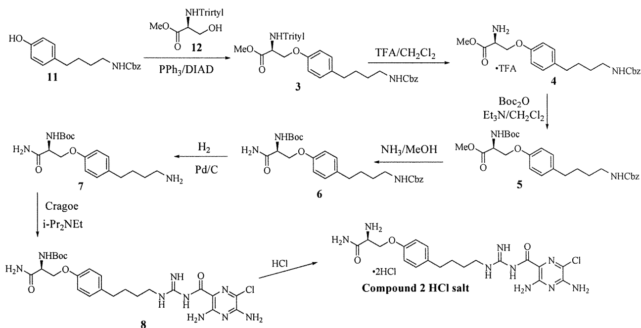
Scheme 1: Synthesis of Compound 2.
