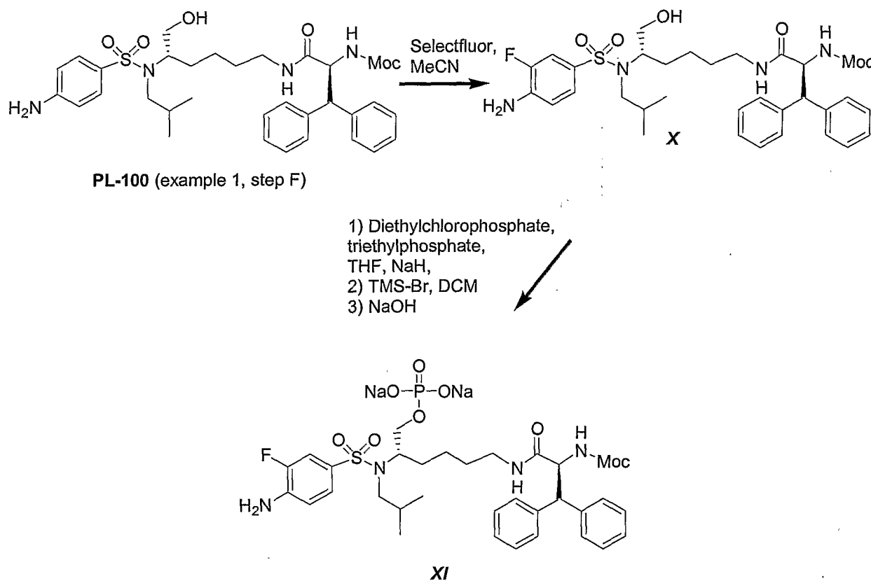
Scheme 3
