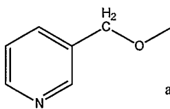
(3-picolyloxy)
