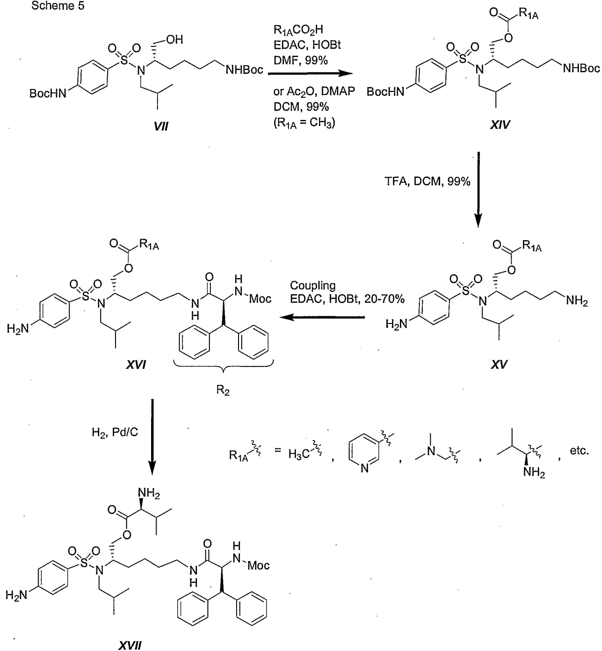
Scheme 5
