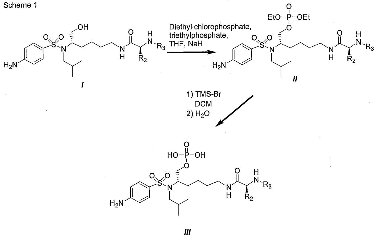
Scheme 1
