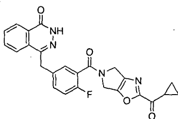
4-(4-fluoro-3-(2-(trifluoromethyl)-4,5,6,6a-tetrahydro-3aH-pyrrolo[3,4-d]thiazole-5-carbonyl)benzyl)phthalazin-1(2H)-one
