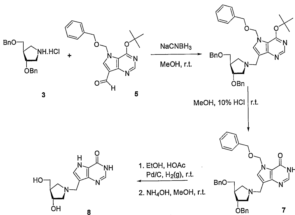
Scheme 3
