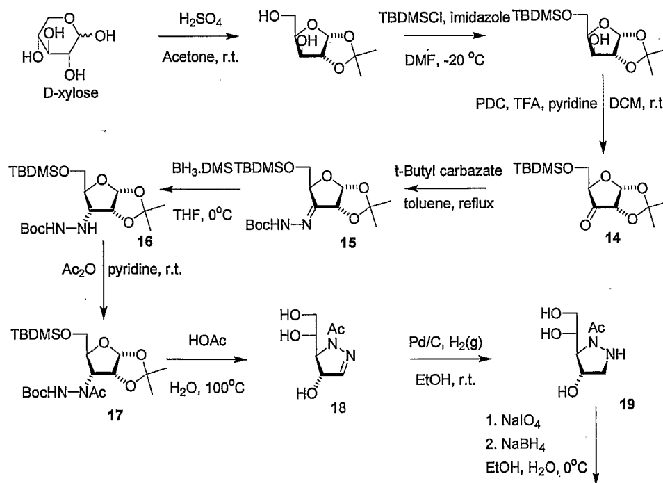
Scheme 6
