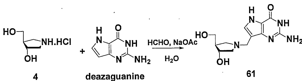
Scheme 17
