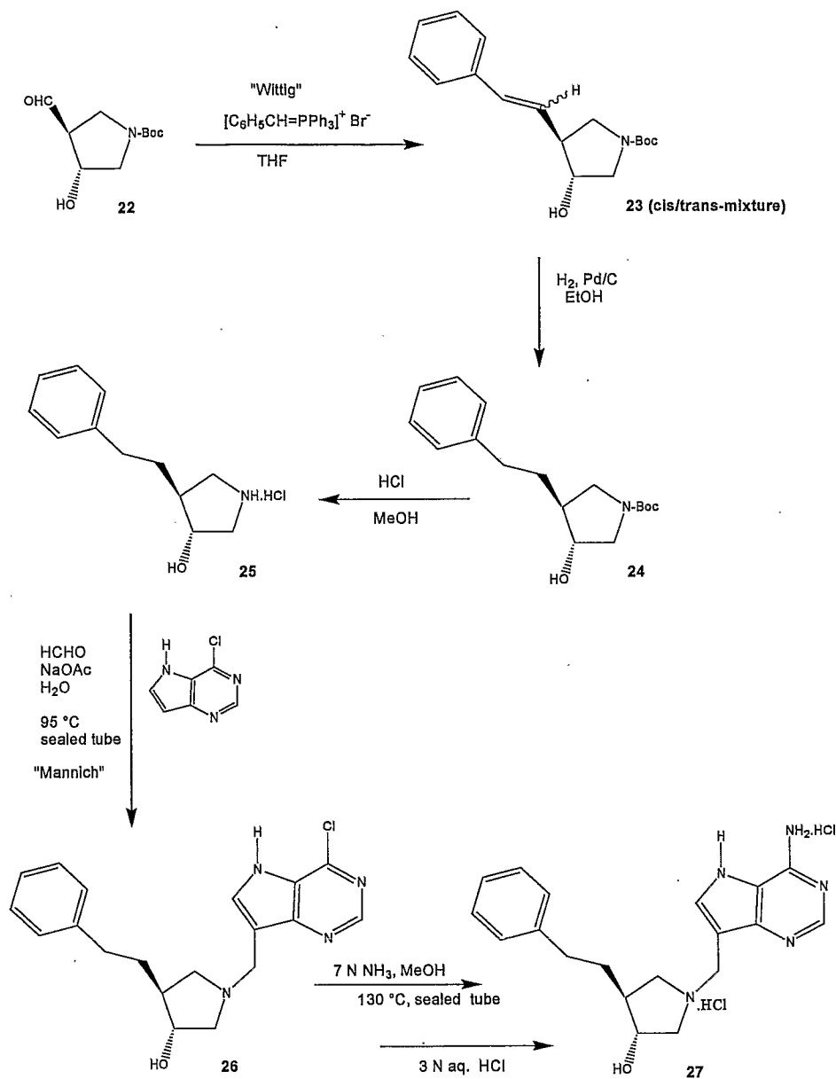
Scheme 7
