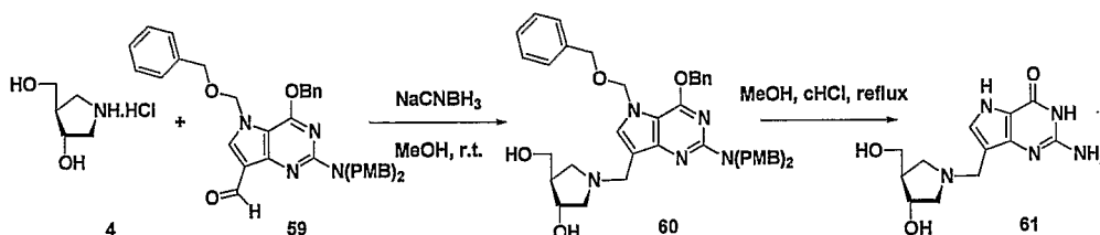
Scheme 16
