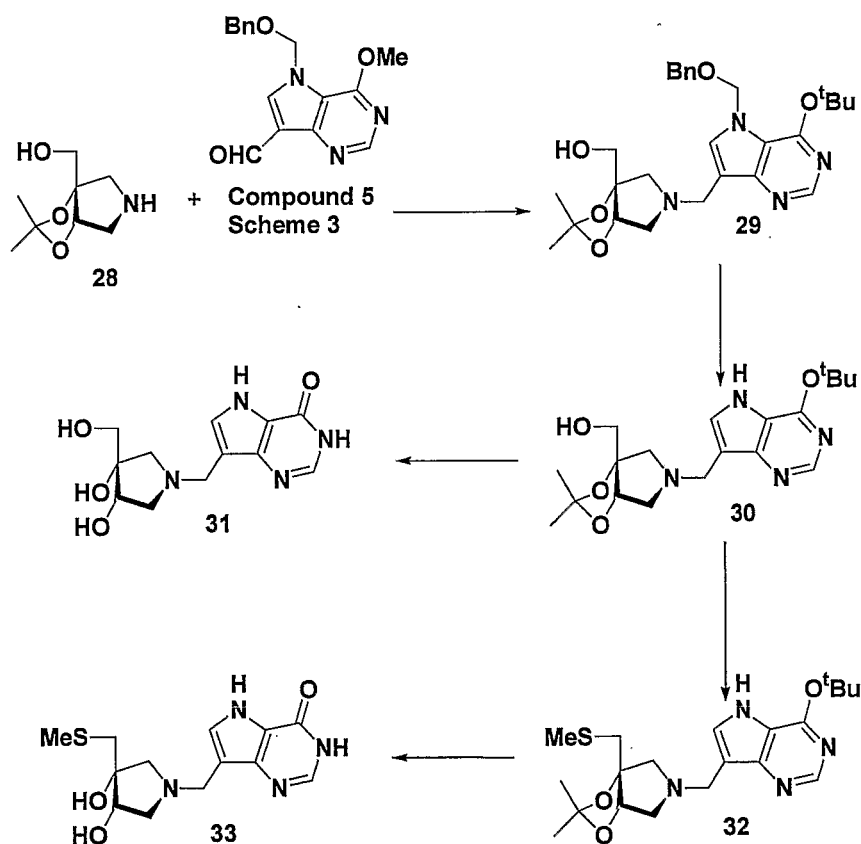
Scheme 9
