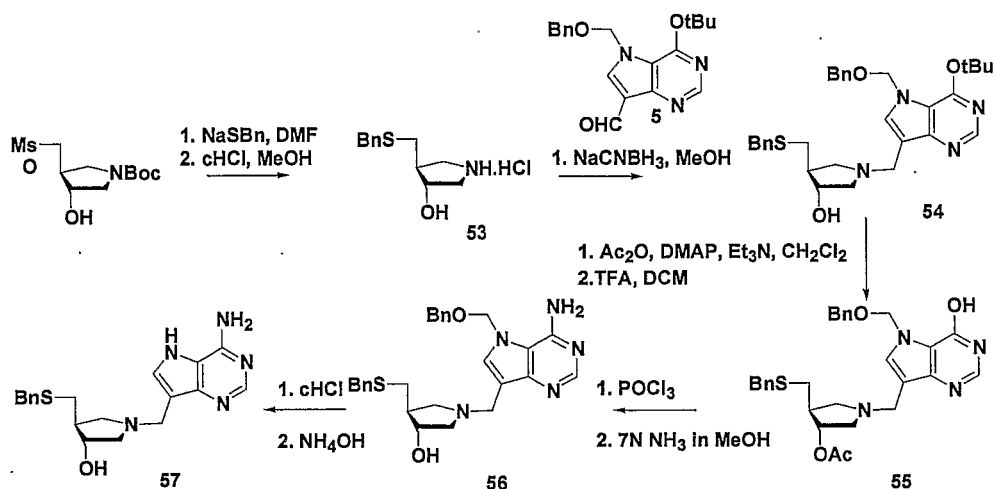
Scheme 14
