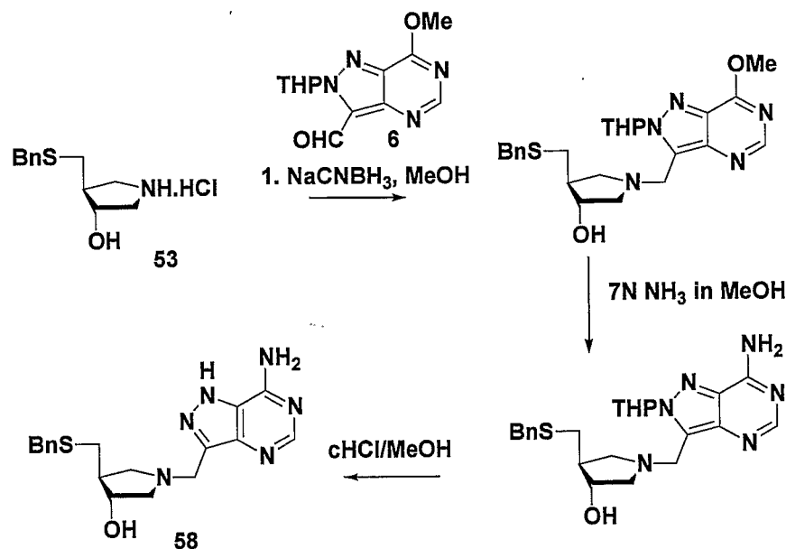
Scheme 15
