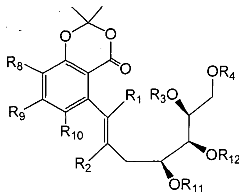
\beta isomer
