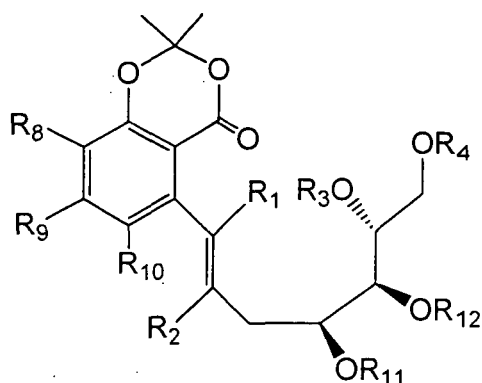
\alpha isomer
