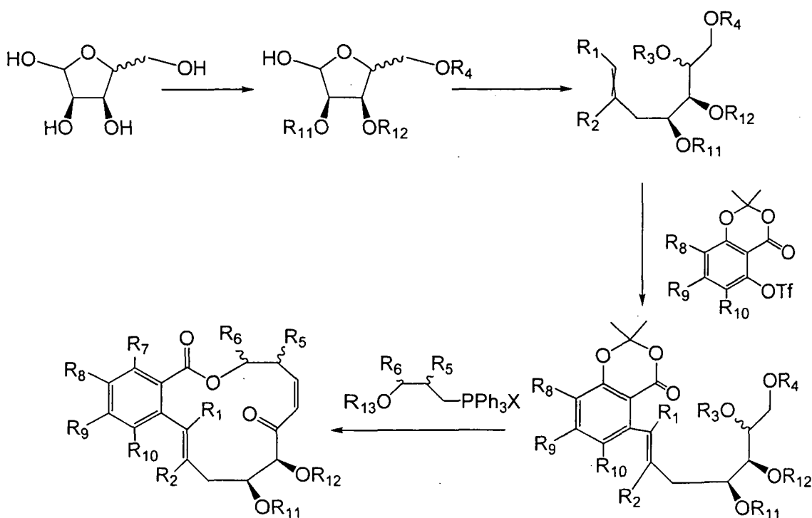
Scheme 2: Synthesis of formula (IV) from ribose – route 2
